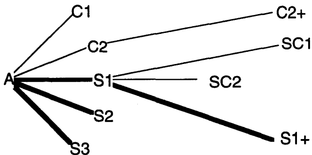
FIGURE 1.—Evolutionary history of the \phi X174 lineages. Branch lengths reflect the duration of propagation (all lineages were grown for either 11 or 22 days); letters indicate isolates. Hosts were either S. typhimurium (thick lines) or E. coli C (thin lines).
