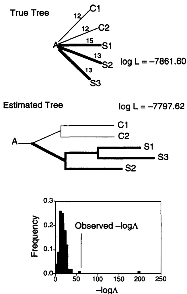
FIGURE 3.—(Top) True history of the five primary \phi X 174 lineages relative to ancestor A. All lineages were grown for 11 days. The numbers on each branch represent the numbers of substitutions occurring throughout the 5386-base genome along each lineage. Log likelihood is for the maximum likelihood reconstruction when the data are forced to obey the true topology. (Middle) Estimated topology and its log likelihood. (Bottom) The distribution of the likelihood ratio statistic, which compares the fit of the data to the true tree vs. the fit of the data to the best-fit tree. The observed ratio lies outside 99% of the distribution, indicating that the true tree is not an acceptable fit to the data.
