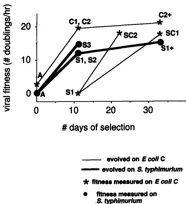
FIGURE 2.— \phi X 174 fitness at 42°. Dots and stars give average fitnesses of the isolates from different lineages. Some points represent two isolates, where the two values are too similar to be viewed separately. *, Fitness assays on host E. coli C ; ●, fitness assays on S. typhimurium . Lines connect ancestors with descendants: heavy lines, growth on S. typhimurium ; thin lines, growth on E. coli . The isolate S1 had very different fitnesses on the two hosts.
