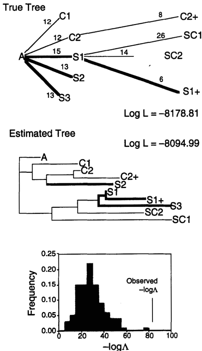
FIGURE 4.— (Top) True history of the nine \phi X 174 lineages relative to ancestor A. Lineages were grown for 11 or 22 days. The numbers on each branch represent the numbers of substitutions occurring throughout the 5386-base genome along each lineage. Log likelihood is for the maximum likelihood reconstruction when the data are forced to obey the true topology. (Middle) Estimated topology and its log likelihood. (Bottom) The distribution of the likelihood ratio statistic, which compares the fit of the data to the true tree vs. the fit of the data to the best-fit tree. Again, the likelihood ratio test rejects the true tree at the 1% level.
