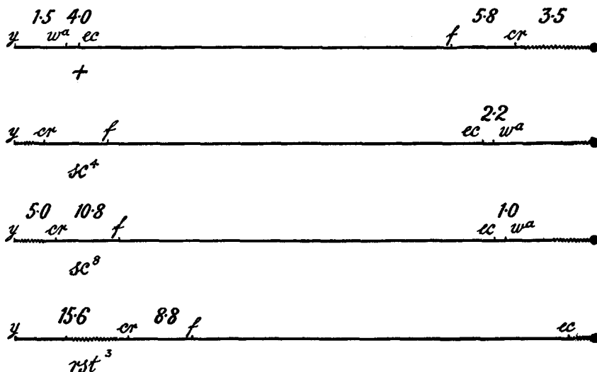
FIGURE 2.—Diagram to illustrate the "spindle fibre" effect. The solid line indicates euchromatin and the wavy line heterochromatin. The numbers above the symbols are the recombination percentages observed.
