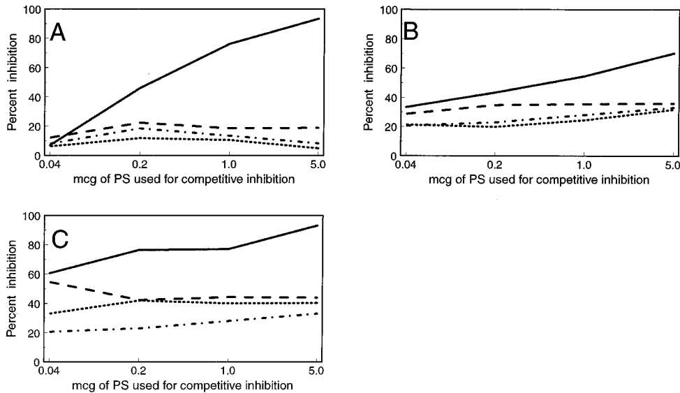
FIG. 5. Effect of PS coating conditions on the specificity of IgG antibodies to the type 3 pneumococcal PS in reference serum 89SF. The serum was used at a dilution of 1:200 and was examined for type specificity following attachment of type 3 PS to the plate by one of the following three methods: precoating of the ELISA plate with 5 µg of mHSA per ml for 6 h and then addition of 5 µg of PS per ml (A), comixing of 1 µg of mHSA per ml with 5 µg of PS per ml (B), and direct coating of 5 µg of PS per ml without mHSA (C). In each method, the antibodies were competitively inhibited by type 3 PS (solid line), type 1 PS (dotted line), type 2 PS (dashed and dotted line), or type 4 PS (dashed line).
