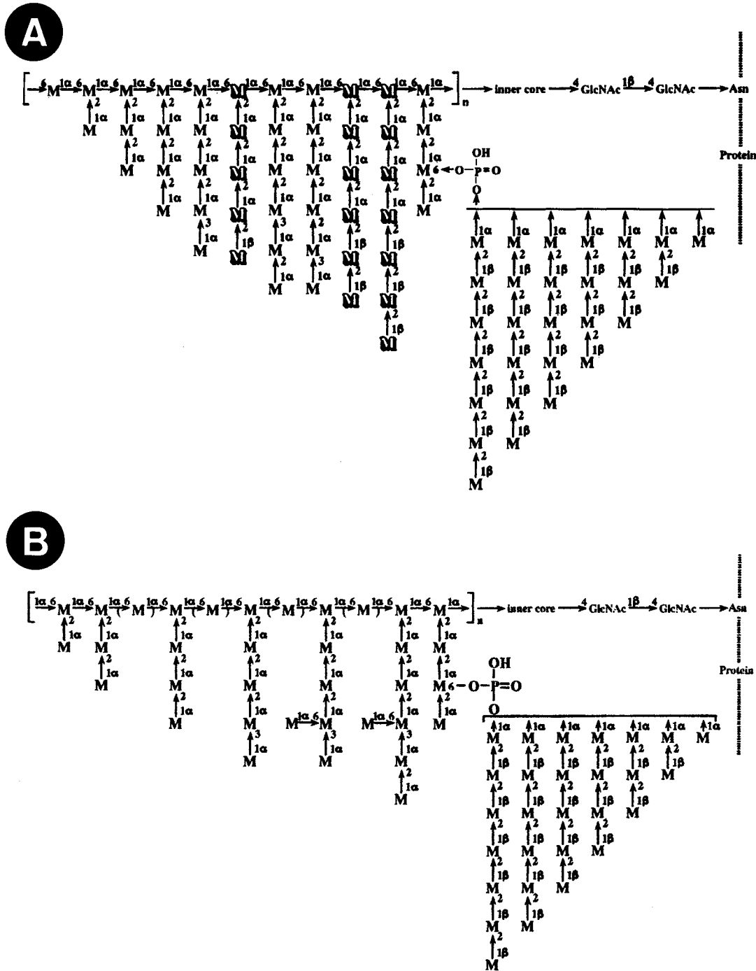
FIG. 1. Structures of C. albicans mannan (M, D-mannopyranose units; GlcNAc, N-acetylglucosamine units; Asn, asparagine residue). (A) Representative structure of serotype A strain mannan. Side chains shown by the outlined letter M indicate putative serotype A-specific structures containing \beta -1,2-linked mannopyranosyl residues at the nonreducing terminal (i.e., antigenic factor 6); other side chains depicted are common in mannans from both serotypes. Reprinted from reference 267 with permission of the publisher. (B) Representative structure of serotype B strain mannan. Single mannose units linked by \alpha -1,6 bonds to the oligosaccharide branches containing \alpha -1,2- and \alpha -1,3-linked mannopyranosyl residues make a serotype B-specific epitope (i.e., antigenic factor 4); \alpha -1,6-linked mannose residues in brackets indicate the partial absence of these units in mannan from C. albicans B cells. Reprinted from reference 271 with permission. Structures corresponding to other antigenic factors present in mannans from both C. albicans serotypes are described in the text.
