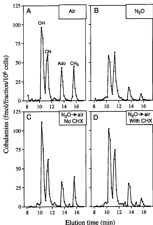
Figure 4 HPLC elution profile of OHCbl (OH), cyanocobalamin (CN), AdoCbl (Ado) and \text{CH}_3\text{Cbl} ( \text{CH}_3 ) in glioma cells exposed to nitrous oxide and during recovery after nitrous oxide exposure
