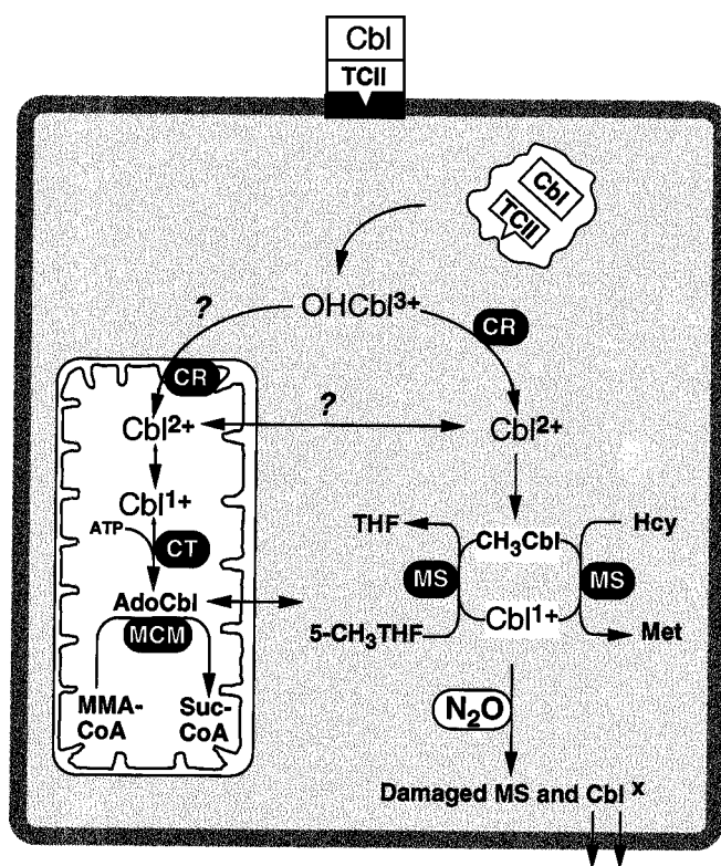
Scheme 1 Interference from nitrous oxide with Cbl metabolism and function
