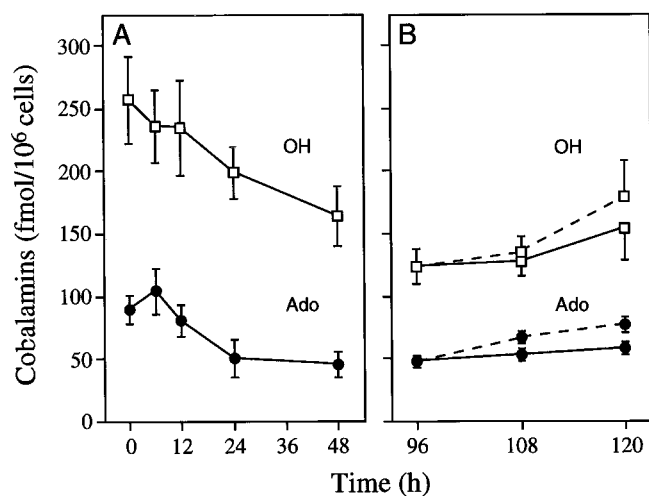
Figure 3 Co-variation of OHcbl and AdoCbl
