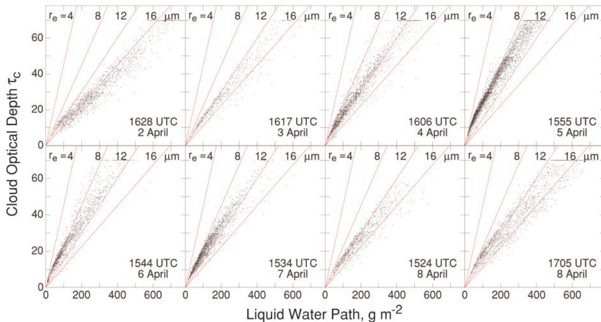
Fig. 3. Pixel-average cloud optical depth \tau_c as a function of vertical cloud LWP for eight satellite overpasses over the study area 50–55°N, 25–30°W, for April 2–8, 1987. Data points with \tau_c > 70 are plotted at \tau_c = 70 because of insensitivity of retrieval method at high optical depth; these points are evident as horizontal clusters at \tau_c = 70 . Data points with \tau_c \leq 3 have been excluded to eliminate pixels that could be covered by haze but not clouds. Lines denote cloud optical depth for indicated constant values of effective radius near cloud top, r_e .
