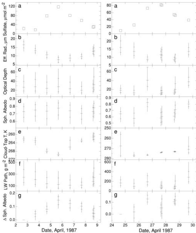
Fig. 2. Time series of sulfate column burden from chemical transport model and pixel-average ( 1 \times 4 km) cloud properties determined from satellite retrievals over mid-North Atlantic, 25\text{--}30^\circ\text{W} , 50\text{--}55^\circ\text{N} , April 2–8, 1987 (Left), and 20.25\text{--}23.625^\circ\text{W} , 43.875\text{--}47.25^\circ\text{N} , April 24–29, 1987 (Right). (a) Modeled sulfate column burden, obtained by interpolation of model output at 6-h intervals. (b) Effective radius at cloud top, r_e . (c) Optical depth, \tau_c . (d) Cloud-top spherical albedo, \alpha_{\text{sph}} . (e) Cloud-top temperature (note inverted scale). (f) LWP. (g) Enhancement of cloud-top spherical albedo relative to that calculated for April 2 (Left) or April 24 (Right) for the same LWP distribution. Bars denote central 80% of the data; ticks denote upper, median, and lower quartiles. Two sets of data are shown for April 8, 27, and 28, for which the study area was within range of the satellite on two successive overpasses. Dates and times are Universal Time Coordinated.
