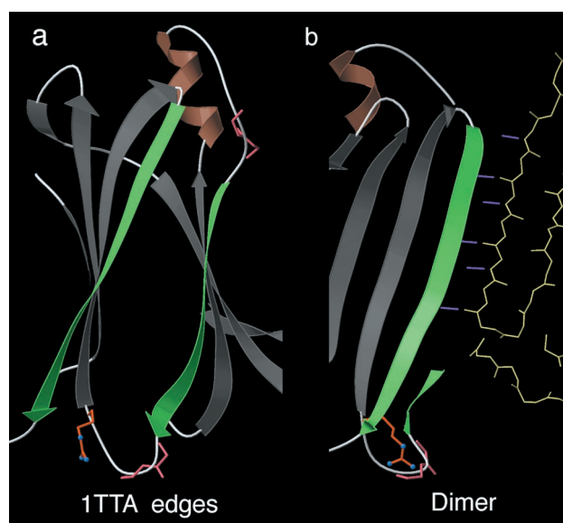
Fig. 5. Edge \beta strands and dimer contacts for the 1TTA transthyretin \beta -sandwich structure (34). (a) Edge strands (green arrows) in the monomer, with a protective charged Arg and two loops (main chain in pink) only at the extreme ends, and long central stretches of completely regular \beta strand, especially on the longer strand at left. (b) That longer edge strand in its dimer contact, with six intersubunit \beta H-bonds (view rotated 90^\circ from a). The shorter edge strand contact (behind; not shown) fits less well, with one H-bond at each end and bridging waters in the center.
