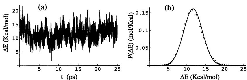
FIGURE 5 (a) Energy gap \Delta E(t) for bR 568 ; (b) distribution of \Delta E(t) values. The dots represent the distribution sampled from (a); the line shows a least squares fit to distribution (2).
