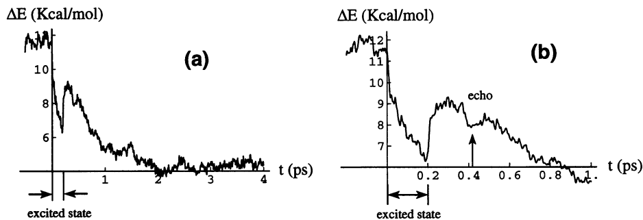
FIGURE 8 (a) The energy gap function \Delta E(t) for bR after photoexcitation in the case that an all trans \rightarrow 13- cis photoisomerization has been induced (see text). The energy gap function has been averaged over 50 trajectories. The excited state charge distribution and the isomerization force field are applied for 0 < t < 200 fs. (b) Same as (a) except for a stretched timescale to reveal details at t \approx 420 fs, i.e., the time at which a dipole echo is expected.
