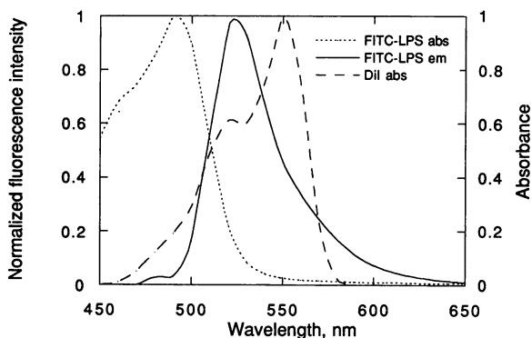
FIGURE 4 Spectral overlap of FITC-LPS and C18-DiI. The absorbance spectrum of 30 ng/ml FITC-LPS from S. minnesota Re 595 (· · ·), fluorescence emission intensity of 30 ng/ml FITC-LPS from S. minnesota Re 595 (—), and the normalized absorbance spectrum of C18-DiI at one molecule per micelle (— —), all in 100 \mu M SBP, 0.02 M TRIS, 0.15 M NaCl buffer at pH 7.5 at 20°C, is shown. The FITC-LPS was excited at 470 nm and the fluorescence peak was normalized to 1.0.
