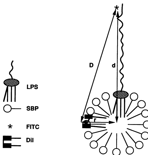
FIGURE 2 Micelle resonance energy transfer model. The SBP detergent micelle is shown with a radius of \sim 20 \text{ \AA} , FITC-labeled polysaccharide linked to a lipid A molecule (LPS) as donor, and a micelle-partitioned C18-DiI as acceptor ( R_o = 68 \text{ \AA} ).
