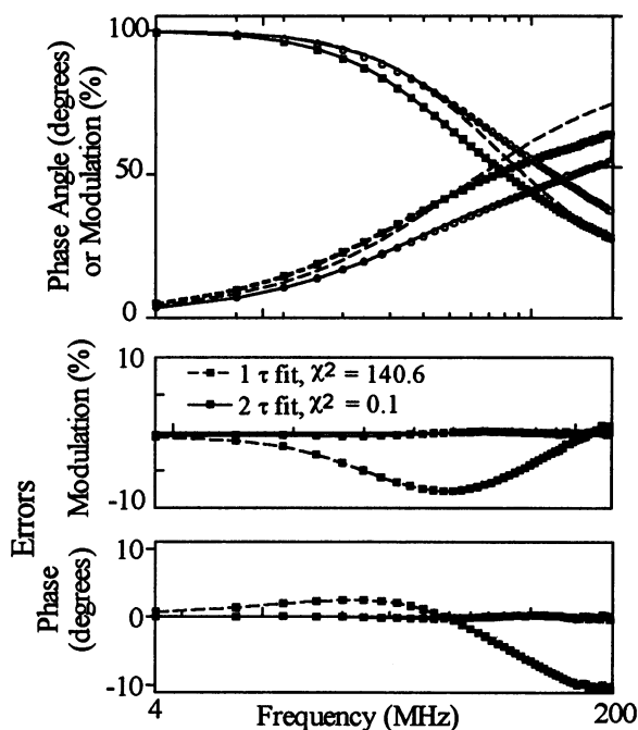
FIGURE 6 Fluorescence lifetime analysis. (Top) Frequency response of donor FITC-LPS from S. minnesota Re 595 native aggregates (O) and after solubilization in 100 \mu M SBP (■) at 20°C, in 0.02 M TRIS, 0.15 NaCl buffer at pH 7. The data are fitted to a two-component lifetime model. A single-lifetime component fit of FITC-LPS S. minnesota Re 595 in detergent is shown (- - -). (Middle) Residual error of lifetime modulation for one-component fit (- - -) and the two-component lifetime fit (—) to the frequency response of native FITC-LPS S. minnesota Re 595 after solubilization in SBP. (Bottom) Residual error of frequency response to phase angle in degrees in FITC-LPS S. minnesota Re 595 upon solubilization in SBP.
