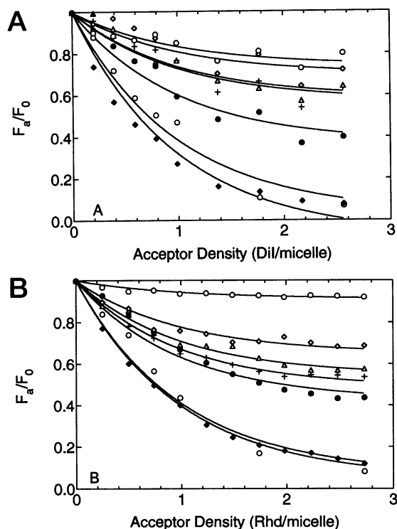
FIGURE 5 Quenching of C18-fluorescein and FITC-LPS in micelles by FRET to acceptors. (A) C18-DiI. (B) C18-Rhd. Data are shown as relative fluorescence ( F_a/F_0 ) versus number of acceptors per micelle. Emission was at 520 nm from different strains of FITC-LPS (30 ng FITC-LPS/ml); excitation wavelength was 470 nm. The FRET data for the FITC-LPS and C18-fluorescein were corrected for quenching of free fluorescein as donor. \blacklozenge , S. minnesota Re 595; \circ , S. minnesota ; \diamond , S. typhimurium ; \bullet , S. abortus equi ; + , Se. marcescens ; \triangle , E. coli 0111:B4; dotted circle, C18-fluorescein; in 100 \mu M SBP at 20°C with 0.02 M TRIS, 0.15 M NaCl buffer at pH 7.5. Energy transfer efficiencies for C18-DiI and C18-rhodamine, respectively, were found by fitting the data with Eq. 7 ( S. minnesota , 0.26, 0.09; S. typhimurium , 0.30, 0.35; E. coli 0111:B4, 0.42, 0.46; Se. marcescens , 0.43, 0.52; S. abortus equi , 0.63, 0.58; C18-fluorescein, 0.97, 0.93; S. minnesota Re595, 1.07, 0.95).
