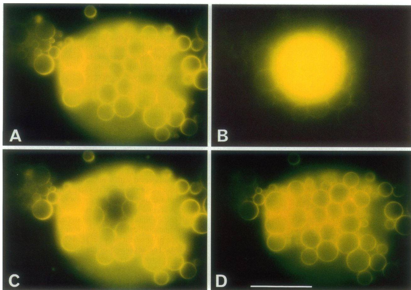
FIGURE 2 EPC liposomes containing 5% of fluorescent phospholipids (NBD-PC). (A) End of the swelling period. (B) A selected area corresponding to a circular domain of 30 \mu\text{m} diameter is illuminated with a laser beam for 1 s. (C) Immediately after illumination, a bleached domain is visible. (D) Two minutes after the bleach, the fluorescence appears to be homogeneously distributed, indicating a diffusion of the fluorescent phospholipids from vesicles to vesicles. The bar corresponds to 30 \mu\text{m} .
