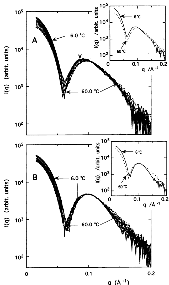
FIGURE 1 Variation of the scattering curve of G_{M1} aggregates in phosphate buffer at pH 6.8. The variation depends on temperatures from 6 to 60^\circ\text{C} . A, at the first temperature scan; B, at the second temperature scan. Thick and dotted lines correspond to the scattering curves of 6^\circ\text{C} and 60^\circ\text{C} , respectively. Insets in A and B extract two curves of both these temperatures. Ganglioside concentration is 0.5% w/v.
