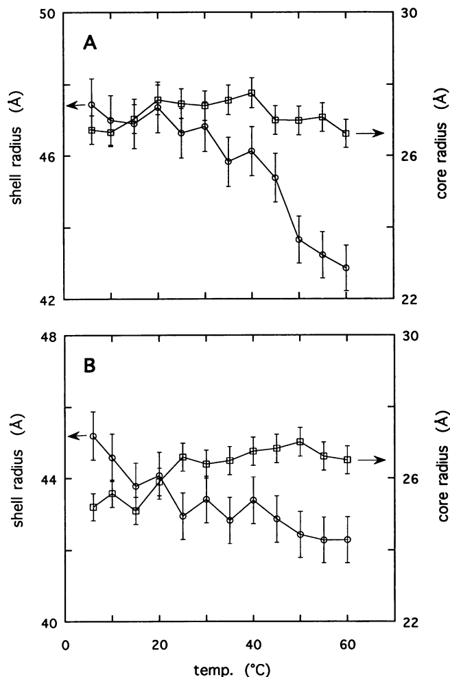
FIGURE 6 Shell and core radii of the ganglioside micelle estimated by the shell-modeling analysis in Fig. 4, plotted against temperature. \circ and \square are the shell and core radii; A and B as in Fig. 1.
