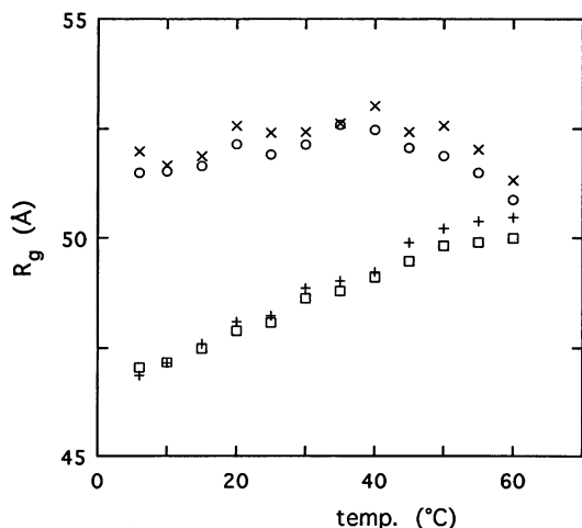
FIGURE 2 Temperature dependence of the gyration radius of the G_{M1} micelle determined by using the Glatter method in Figs. 1 and 3. \circ , for the first temperature scan; \square , for the second temperature scan. \times and + correspond to the gyration radii for the first and second scans obtained from the modeling analysis in Figs. 4 and 5.
