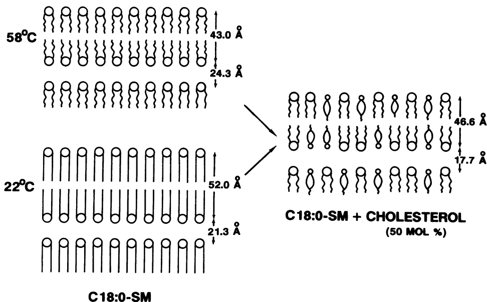
FIGURE 11 Summary of the structural changes exhibited by C18:0-SM (left) on incorporation of 50 mol% cholesterol (right).
