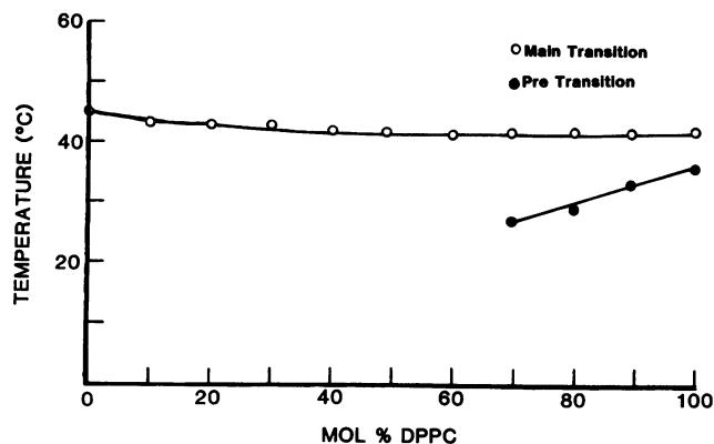
FIGURE 9 Plot of transition temperature of hydrated (75 wt% water) C18:0-SM/DPPC mixtures. \circ , Chain-melting transition; \bullet , pre-transition.
