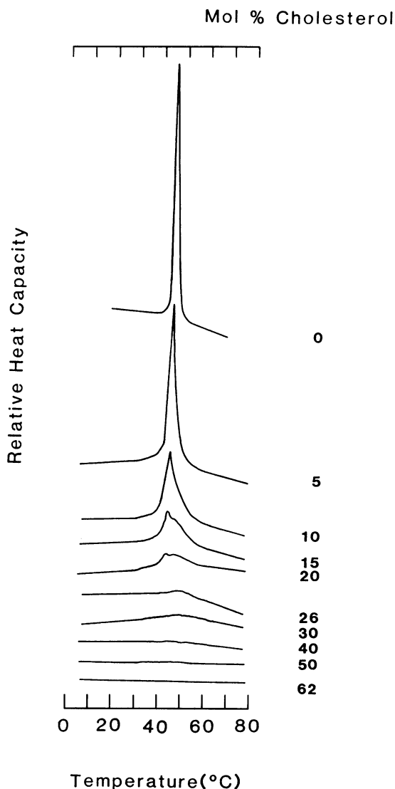
FIGURE 3 DSC heating scans of fully hydrated (75 wt% water) C18:0-SM containing 0, 5, 10, 15, 20, 26, 30, 40, 50 and 62 mol% cholesterol. Heating scan rate, 5^\circ\text{C}/\text{min} .
