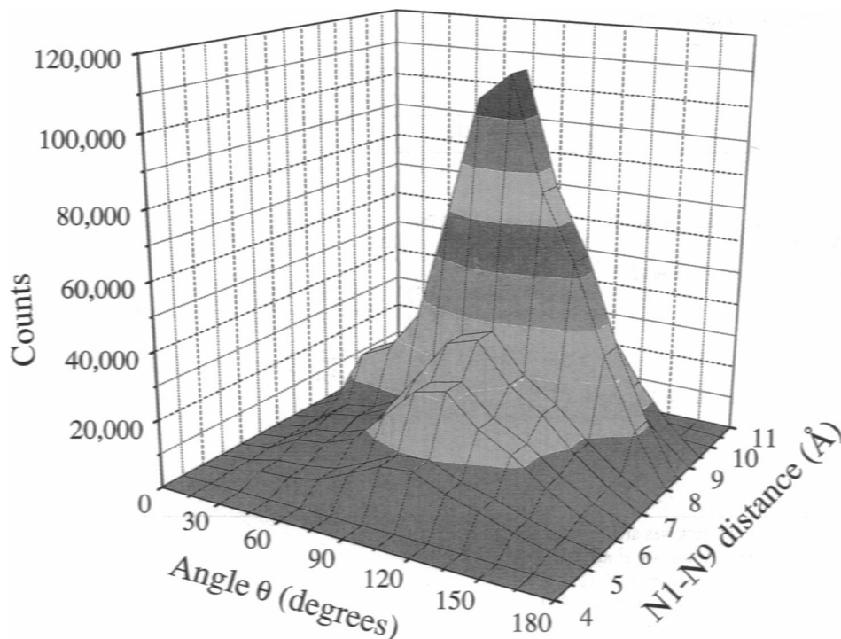
FIGURE 10 Conformational probability distribution as a function of the N1-N9 distance and the angle between the base plane normals for the unstacked MD simulation.
