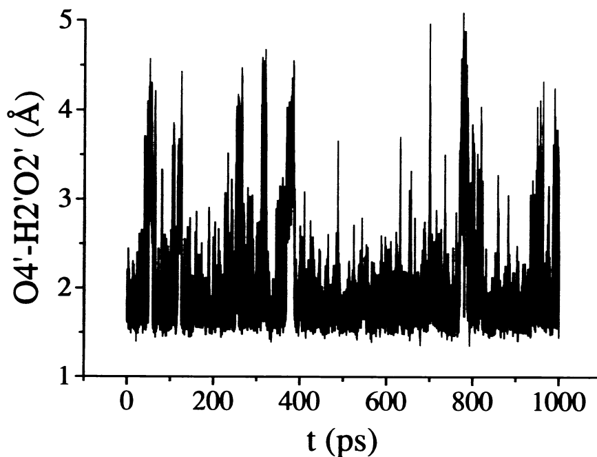
FIGURE 11 The time evolution of the O4'...H2'-O2' hydrogen bond of the stacked conformation.
