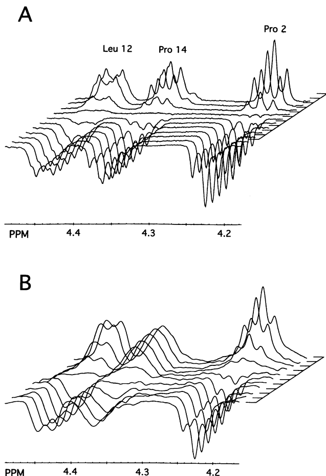
FIGURE 2 ^1H NMR spectra showing the time-dependent magnetization of the C\alpha protons of Leu12, Pro 14, and Pro 2 as measured by the inversion-recovery sequence 180-t-90-acquisition, as a function of \tau , where \tau = 1 \mu s , 1, 20, 50, 100, 200, 500, 800 ms, and 1.2, 3.0, 5.0 s. In (A) spectra for 2 mM native alamethicin in methanol; in (B) spectra for 2 mM alamethicin with a proxyl spin label attached to the C-terminus in methanol.
