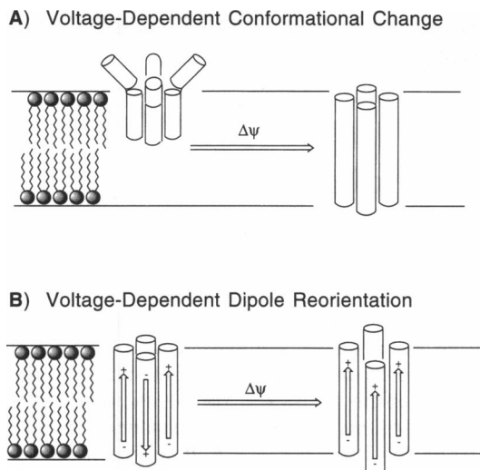
FIGURE 1 A number of mechanisms have been proposed to account for the voltage gating of alamethicin that require quite different properties of the peptide monomer. For example, (A) shows a model involving a voltage-dependent conformational change in alamethicin that leads to the membrane insertion of an aggregate (Fox and Richards, 1982); (B) shows a model that involves the voltage-dependent reorientation of the alamethicin helix, leading to electrostatic repulsion in the aggregate and an opening of the channel (Boheim et al., 1983; Mathew and Balaram, 1983).
