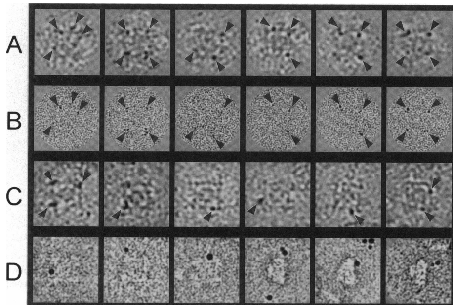
FIGURE 3 Selected images from electron micrographs of gold cluster-CaM-treated RyR. (A) Frozen-hydrated Au 1.4-nm -CaM:RyR complexes prepared using Au 1.4-nm -CaM prepared by method I (see Materials and Methods). Micrograph recorded with objective lens underfocused by 1.5 \mu\text{m} . (B) Same RyRs as in A except recorded at 0.5 \mu\text{m} underfocus to contrast the gold clusters. (C) Selected images of Au 1.4-nm -CaM:RyR complexes prepared using Au 1.4-nm -CaM prepared by method II (see Materials and Methods). Recorded at 1.5 \mu\text{m} underfocus. (D) Negatively stained biotinylated CaM:RyR complexes treated with streptavidin-colloidal gold (5 nm diameter gold). The first three frames show RyRs in fourfold symmetric orientation, and last three show receptors in orientation approximately normal to the fourfold symmetry axis. Underfocus, \approx 0.5 \mu\text{m} . The width of each frame in A–D is 64 nm. Arrowheads denote positions of gold clusters.
