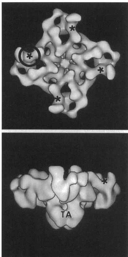
FIGURE 5 Locations of bound Au_{1.4\text{-nm}} -CaM in three dimensions. The positions of the bound gold clusters were inferred by projecting their locations in the two-dimensional averaged Au_{1.4\text{-nm}} -CaM:RyR complex (Fig. 4 B) onto the cytoplasmic face of the three-dimensional reconstruction of frozen-hydrated RyR reported by Radermacher et al. (1994). The top image shows the RyRs cytoplasmic face viewed parallel to the fourfold symmetry axis. The gold cluster locations are indicated by asterisks; one of the sites is centered within a circle of radius equal to 4 nm to indicate the area within which the center-of-mass of the CaM must lie (see Discussion). The bottom image shows a side view of the RyR (i.e., a view perpendicular to the fourfold symmetry axis) with one of the gold cluster locations denoted by an asterisk. TA, transmembrane assembly.
