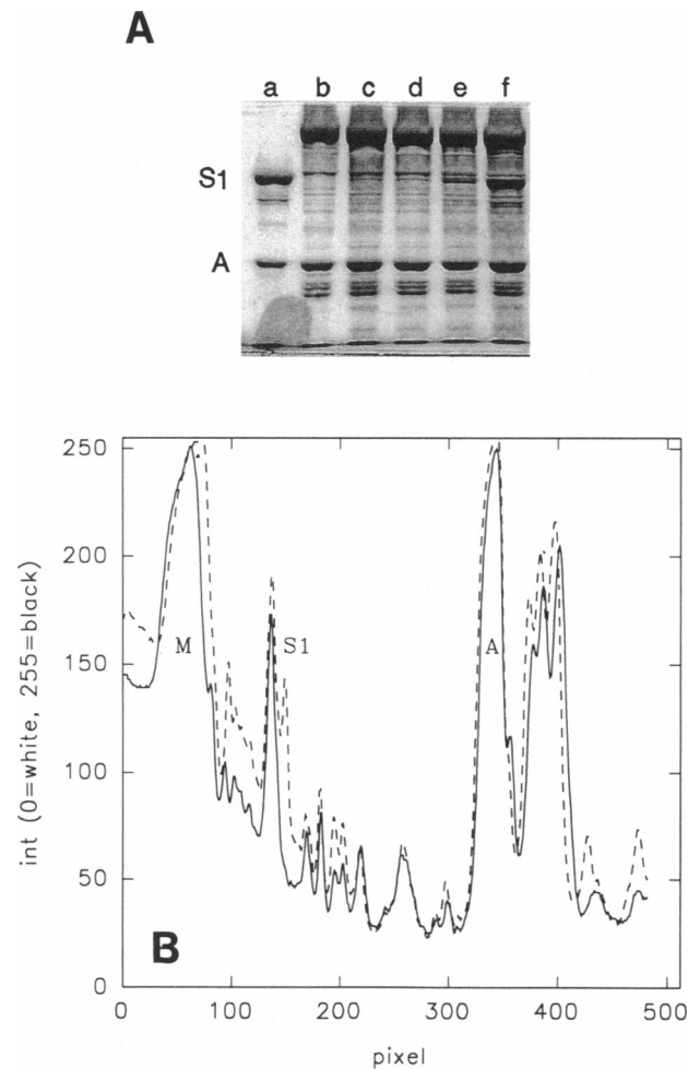
FIGURE 4 In A, SDS-PAGE pattern of myofibrils irrigated with increasing concentrations of S1. (a) S1 and actin at molar ratio of 1:1. (b–f) 1 mg/ml myofibrils were incubated with various concentrations of S1 for 40 min at room temperature, centrifuged at 1000 rpm for 5 min, and electrophoresed on SDS-PAGE. (b) Native myofibrils. (c) Myofibrils + 0.02 \mu\text{M} S1. (d) Myofibrils + 0.1 \mu\text{M} S1 (such preparations were used for experiments using "low" concentration of S1). (e) Myofibrils + 0.5 \mu\text{M} S1. (f) Myofibrils + 2 \mu\text{M} S1 (such preparations were used for experiments using "high" concentration of S1). In B, intensity profiles of myofibrils irrigated with 0.1 \mu\text{M} S1 used to measure the molar ratio of S1:actin. The intensities have been reversed and 0 corresponds to white and 255 to black.
