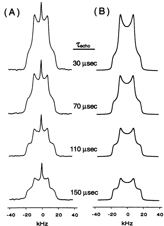
FIGURE 2 ^2\text{H} NMR powder pattern spectra of \text{Ala}_5\text{-d}_4 gramicidin A in hydrated DMPC bilayers. (A) Experimental spectra obtained with 60,000 acquisitions using the quadrupole echo experiment with the various echo delays shown. (B) Spectral simulations for these delay times. Simulations of the global motion were achieved by 10^\circ jumps between 36 sites for the \text{C}_\alpha\text{-C}_\beta axis in a cone of semi-angle 98^\circ . A quadrupole coupling constant of 51 kHz was used and a jump rate of 3.0 \times 10^7 Hz ( \tau_p = 43 \mu\text{s} ) resulted in the best fit to the experimental data.
