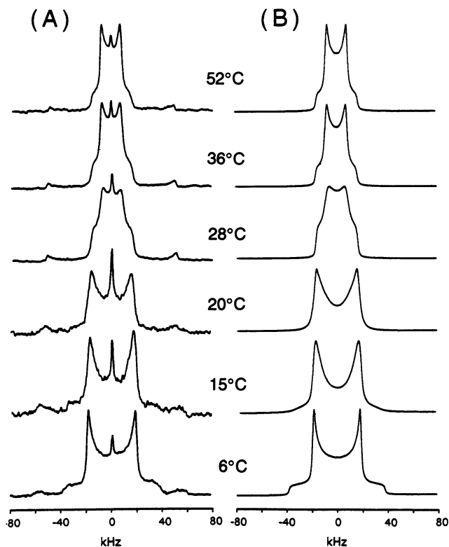
FIGURE 4 Temperature dependence of the Ala_3 - d_4 gramicidin A ^2H powder pattern spectra in hydrated DMPC bilayers. (A) Experimental spectra obtained with 60,000 acquisitions using the quadrupole echo experiment with a 30- \mu s echo delay. (B) Spectral simulations for the various temperatures using the following correlation times: 52°C (325 K), \leq 13 \mu s ; 36°C (309 K), 29 \mu s ; 28°C (301 K), 130 \mu s ; 20°C (293 K), 1.3 ms; 15°C (288 K), 4.3 ms; 6°C (279 K), \geq 1.3 s .
