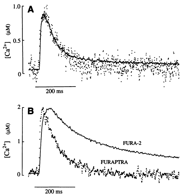
FIGURE 5 Comparison of the time course of [Ca^{2+}]_i transients measured with furaptra (dots) and two fura-2 (solid lines) concentrations. [Ca^{2+}]_i transients were elicited by 50-ms depolarizations from -70 to +10 mV. Cells were loaded with furaptra by voltage-clamping with pipettes containing 300 \mu\text{M} indicator. (A) The average [Ca^{2+}]_i transient in cells loaded with low fura-2 concentration ( 10 \mu\text{M} in the pipette) is scaled by a factor of 2.1 to match the peak of furaptra [Ca^{2+}]_i transient and superimposed on the average transient in furaptra-loaded cells (same data as Fig. 4). (B) Average [Ca^{2+}]_i transients calculated from three cells loaded with fura-2 ( 50 \mu\text{M} in the pipette) and four cells loaded with furaptra. The average [Ca^{2+}]_i transient of the fura-2-loaded cells is scaled by a factor of 6.4 to match the peak for the average transient in furaptra-loaded cells.
