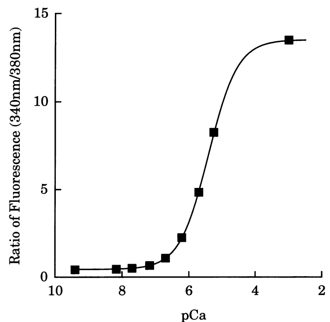
FIGURE 1 In vitro calibration of fura-2. Calibration of fura-2 in a 100-μm diameter glass capillary. The solid line was determined by fitting the data with a nonlinear least squares routine to a sigmoid equation with the following parameters: R_{min} = 0.43 , R_{max} = 13.4 , and K_D \cdot \beta = 3.2 \mu M , Hill coefficient = 1.
