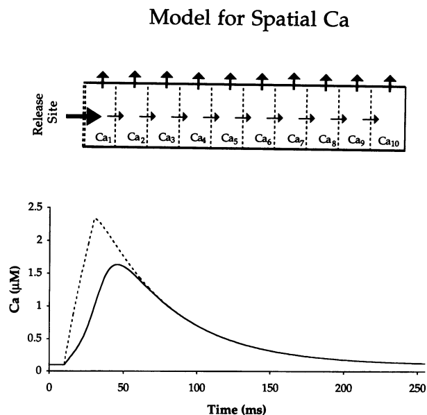
FIGURE 9 Effect of spatial gradients of [\text{Ca}^{2+}]_i on the [\text{Ca}^{2+}]_i transients measured with a low and high affinity indicator. (A) Model half sarcomere. The half sarcomere is modeled as a 10-compartment space where each compartment occupies 0.1 \mu\text{m}^3 . \text{Ca}^{2+} is released only into compartment 1 but is removed from all compartments (see text for details). (B) \text{Ca}^{2+} transients estimated with a low ( K_D = 20 \mu\text{M} ) and high affinity ( K_D = 0.2 \mu\text{M} ) \text{Ca}^{2+} indicator. Superimposed \text{Ca}^{2+} transients are calculated by assuming rapid equilibrium between the indicator and \text{Ca}^{2+} in each compartment for the high affinity (solid curve) and low affinity indicator (dashed line). \text{Ca}^{2+} release (i.e., input into compartment 1) occurs from 10–30 ms at a constant rate ( 1.5 \mu\text{M}/\text{ms} ).
