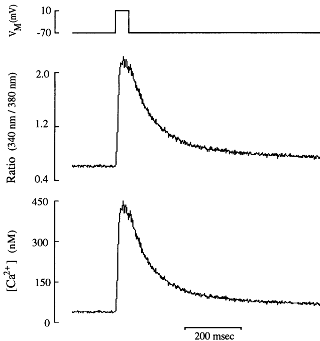
FIGURE 2 [Ca 2+ ] i transient measured with fura-2. The voltage (top), ratio of 500-nm fluorescence intensities (middle), and [Ca 2+ ] i transient (bottom) are shown for a myocyte voltage clamped with an electrode containing 50 \mu M fura-2. The calibration parameters for conversion of ratio to [Ca 2+ ] i are R_{\min} = 0.41 , R_{\max} = 13.0 , \beta = 13.1 , and K_D = 239 nM.
