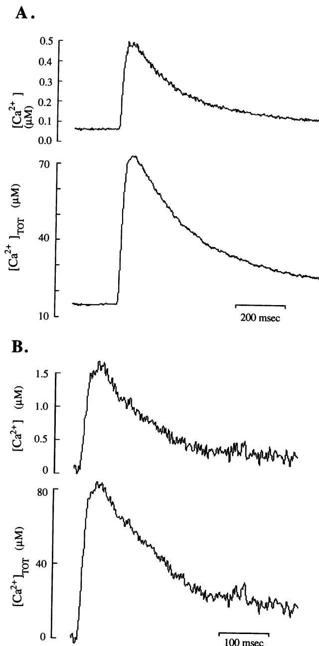
FIGURE 7 Estimation of the moles of Ca^{2+} involved in [Ca^{2+}]_i transients. The top panel is a [Ca^{2+}]_i transient determined in a cell loaded with fura-2 (A) and furaptra (B). The bottom panel is an estimation of the total [Ca^{2+}] participating in the [Ca^{2+}]_i transient shown in the top panel. Total [Ca^{2+}] (in \mu\text{mol/liter} cytoplasmic \text{H}_2\text{O} ) was calculated with a one-compartment model (see text for details) which included the Ca^{2+} buffers listed in Table 2.
