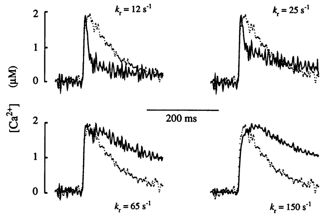
FIGURE 8 Kinetic correction of fura-2 fluorescence signals. Each panel shows the superimposed [Ca 2+ ] i transients which are the average of those determined in four fura-2pr (dashed line) and three fura-2-loaded myocytes (solid line). The fura-2 [Ca 2+ ] i transients were calculated by converting the ratio of fluorescence intensity ( R ) to [Ca 2+ ] i with Eq. A8 where k_{\text{on}} and k_{\text{off}} were arbitrarily chosen so that K_D = 239 nM. The reverse rate constant used in the calculation is shown at the top of each panel. The scale factors are 2.0 ( k_{\text{off}} = 12 s -1 ), 3.1 ( k_{\text{off}} = 25 s -1 ), 6.2 ( k_{\text{off}} = 65 s -1 ), and 6.4 ( k_{\text{off}} = 150 s -1 ). These data are taken from experiments also shown in Fig. 5 B.
