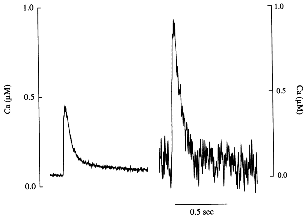
FIGURE 4 Comparison of [Ca 2+ ] i transients in cells loaded with low fura-2 concentrations and fura-2r. [Ca 2+ ] i transients were elicited by 50-ms depolarizations from -70 to +10 mV. The electrode solution contained 10 μM fura-2 (left panel) or 300 μM fura-2r (right panel). The [Ca 2+ ] i transients displayed are the average of [Ca 2+ ] i transients observed in four cells loaded with fura-2 and six cells loaded with fura-2r.
