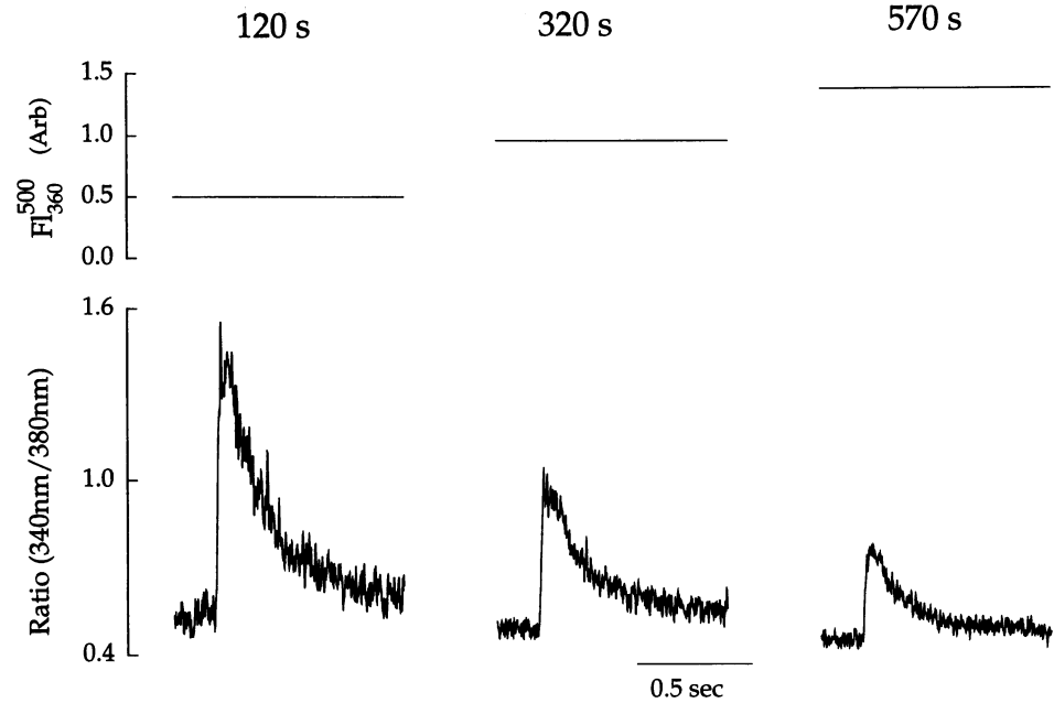
FIGURE 3 Effect of fura-2 loading on the amplitude of the [Ca^{2+}]_i transient. The top panels show the level of fluorescence measured at the isosbestic point, with 360-nm illumination. The time after establishing a whole cell voltage clamp is indicated. The bottom panels show the [Ca^{2+}]_i transient, displayed as the ratio of fluorescence intensity, elicited by 50 ms depolarizations from -70 to +10 mV.
