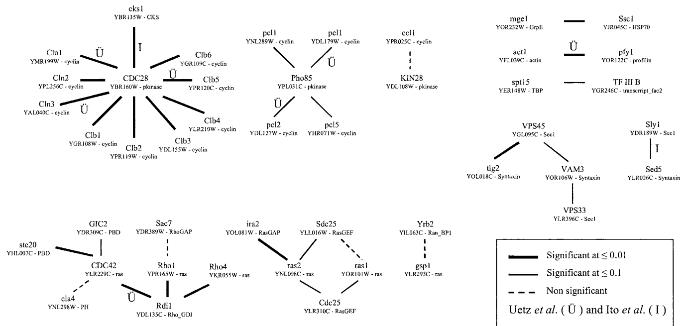
Fig. 3. Yeast interactions mapped onto known 3D complexes. Yeast proteins are given by their YPD names, codes, and Pfam families. Thick lines denote interactions significant at \leq 0.01 , thin lines 0.01-0.1 , and dashed lines > 0.1 .
