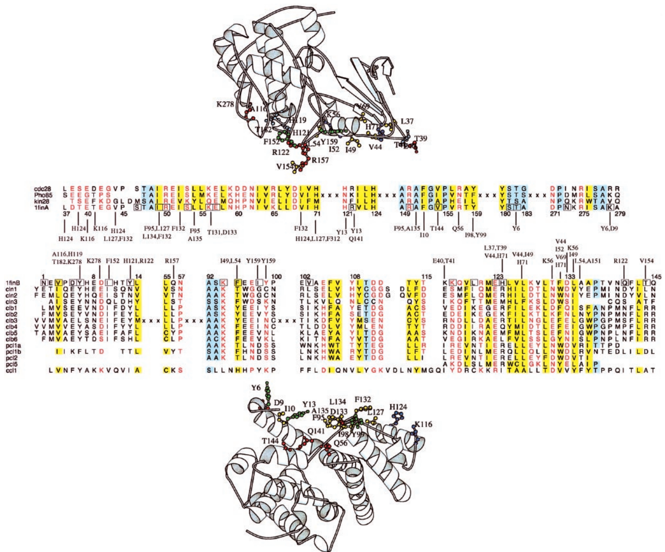
Fig. 4. The kinase/cyclase system in yeast. Sequences are denoted by YPD or PDB codes. The known structure [1fin (35)] is that of human CDK2 (Upper)/cyclin A (Lower). Details are otherwise as for Fig. 2.
