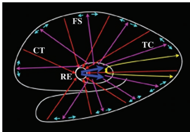
Fig. 4. Thalamocortical model of fast and low-frequency rhythm synchronization. A near midsagittal view of the cortical mantle is shown as the outermost white trace whereas the outer boundary of the thalamus, also in white, is shown near the center of the figure. The RE is also shown within the thalamus. Spatially specific excitatory neurons, shown in yellow, subserve fast rhythm synchronization and make monosynaptic connections via the body of the thalamus. The remaining circuitry subserves low-frequency rhythm synchronization. Spatially widespread excitatory corticothalamic (CT) afferents, shown as red arrows, project to RE. Thick blue arrows indicate inhibitory afferents from RE to TC neurons. Spatially widespread excitatory TC neurons, shown as magenta arrows, project to cerebral cortex and activate fast-spiking (FS) inhibitory cells, shown in cyan.
