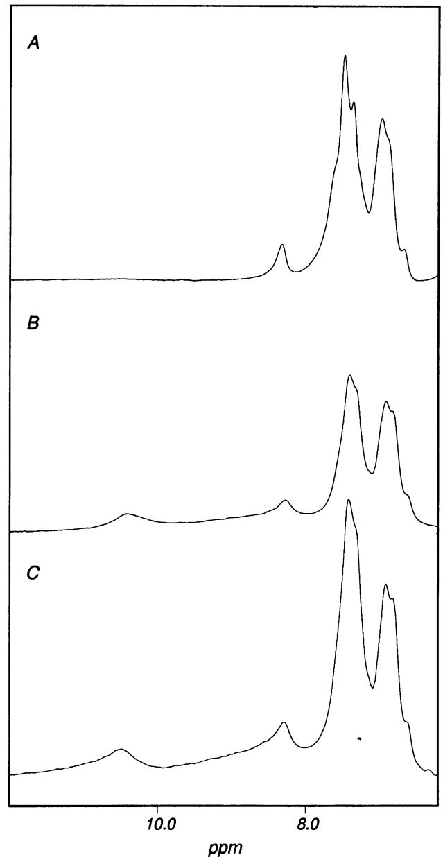
FIGURE 3 MAS ^1\text{H} NMR spectra of gramicidin/DLPC (mole ratio 1:20, lipid concentration 50% w/w) recorded at 50^\circ\text{C} with regioselective excitation of the low-field peptide region in ^2\text{H}_2\text{O} (A), in \text{H}_2\text{O} with presaturation (B), and in \text{H}_2\text{O} with jump-return (C). The intensities of spectra B and C are directly comparable.
