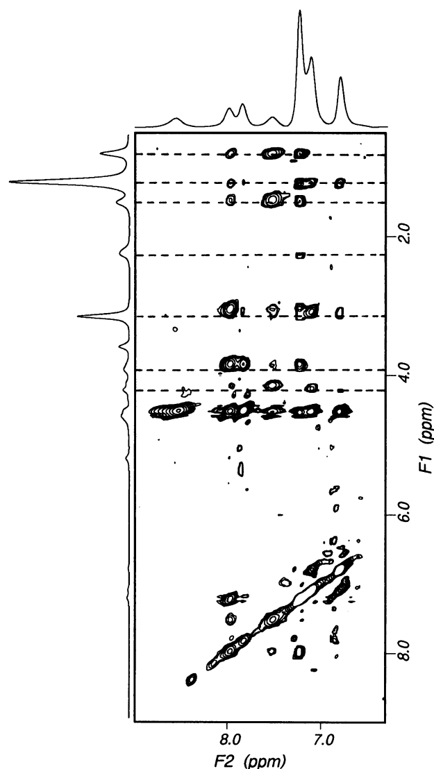
FIGURE 7 Low-field region of the MAS ^1\text{H} F2-regioselective 2D NOESY spectrum of leucine enkephalin/DLPC (mole ratio 1:20, lipid concentration 50% w/w) recorded at 30°C in \text{H}_2\text{O} with jump-return at a mixing time of 400 ms. The corresponding nonselective 1D spectrum is displayed on the left, and the regioselective 1D spectrum is displayed on the top for comparison. The dotted lines correspond to the chemical shifts of the main lipid resonances.
