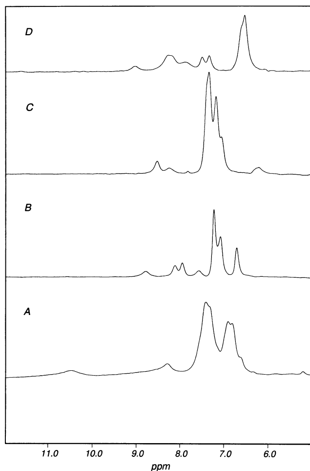
FIGURE 4 MAS ^1\text{H} NMR spectra of (A) gramicidin A/DLPC at 50^\circ\text{C} , (B) leucine-enkephalin/DLPC at 30^\circ\text{C} , (C) zfFG/DMPC at 50^\circ\text{C} , and (D) myr-KRTLRL/DMPC at 40^\circ\text{C} (mole ratio 1:20, lipid concentration 50% w/w) in \text{H}_2\text{O} recorded with regioselective excitation of the low-field peptide region and jump-return.
