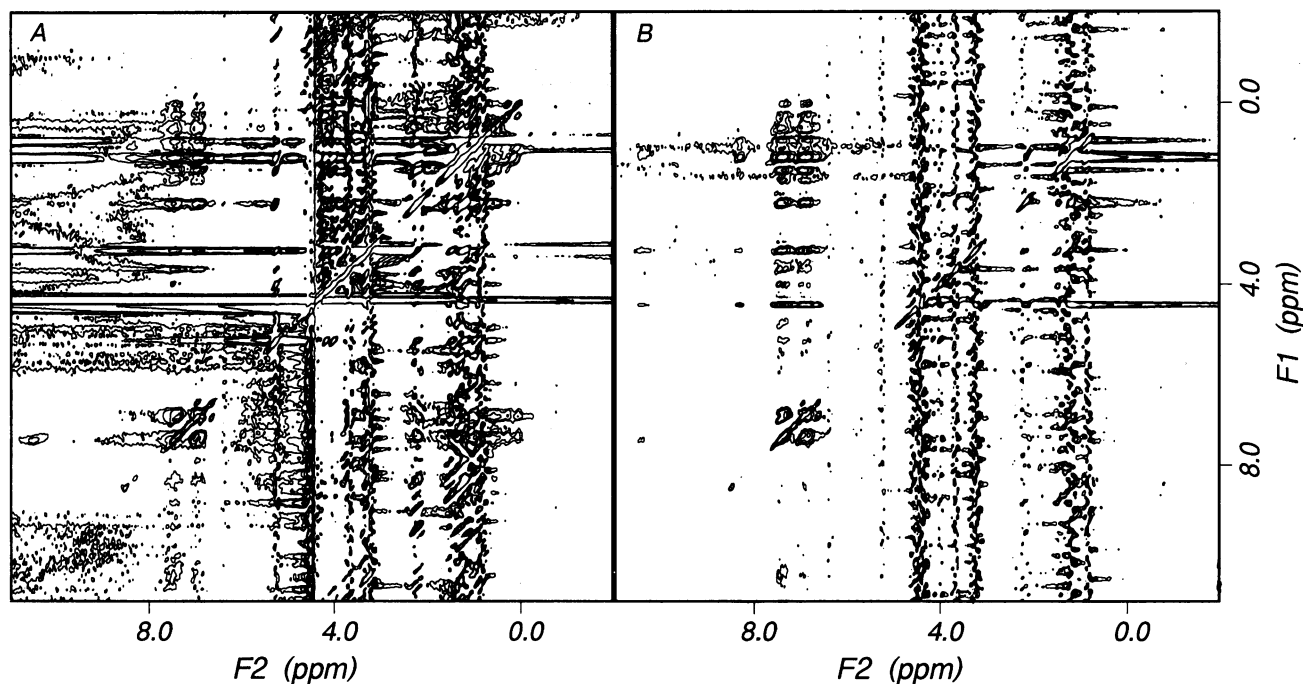
FIGURE 5 MAS ^1\text{H} 2D NOESY spectra of gramicidin/DLPC (mole ratio 1:20, lipid concentration 50% w/w) recorded at 50^\circ\text{C} in \text{H}_2\text{O} with presaturation with (A) classical and (B) F2-regioselective excitation. The mixing time is 200 ms.
