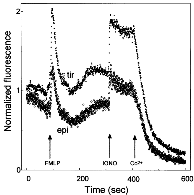
FIGURE 3 FMLP-induced Ca^{2+} transients in bulk cytosol and membrane-proximal regions. Fluo-3-loaded cells were viewed by TIR (●) and EPI (○) during the course of buffer-specific replacements. The first arrow indicates the time of introduction of buffer containing 100 nM of the N -formyl peptide chemoattractant FMLP. At the second arrow the buffer was replaced with buffer containing 26 \mu M ionomycin, the channel-forming drug, which nonspecifically allows extracellular Ca^{2+} to rush into the cell. At the third arrow the buffer was again replaced with 26 \mu M ionomycin and 0.12 mM cobalt ion, which enters the cell through the ionomycin channels and binds and quenches Fluo-3 fluorescence. The photon counting interval here was 100 ms.
