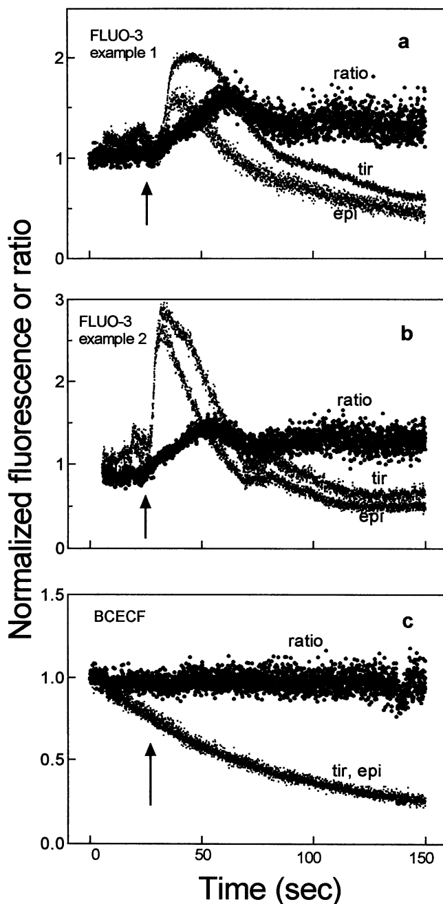
FIGURE 4 (a and b) FMLP-induced transient changes in the membrane-proximal/cytosolic Ca^{2+} ratio. Two examples are shown of Fluo-3-loaded cells activated with 100 nM FMLP added at the arrow. After the addition, a slight delay ensues before the FMLP reaches the cell under view. The individual traces for TIR and EPI are indicated by thin dots, and the ratio of TIR/EPI by thicker dots. (c) Lack of change in the TIR/EPI ratio for the fluorophore BCECF. Cells were loaded with BCECF as described in the text; 100 nM FMLP was added at the arrow. The photon counting interval for these three graphs was 30 ms.
