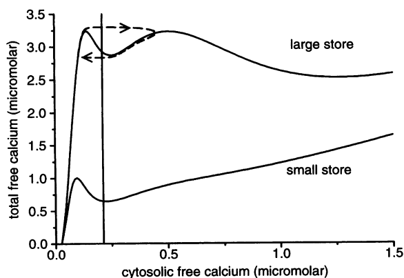
FIGURE 9 Nullclines of the simplified open-cell model for the large and the small stores. The vertical nullcline is for the C_o equation (cf. Eq. 14); the remaining curves are nullclines for the [\text{Ca}_i^{2+}] equation (cf. Eq. 13). For these parameters (the same as for Fig. 8, with j_{in} = 1.0 \mu\text{M s}^{-1} ), the intersection of the nullclines is an unstable steady state. (— — —) The oscillatory trajectory surrounding the unstable state, with arrows showing direction of change in time.
