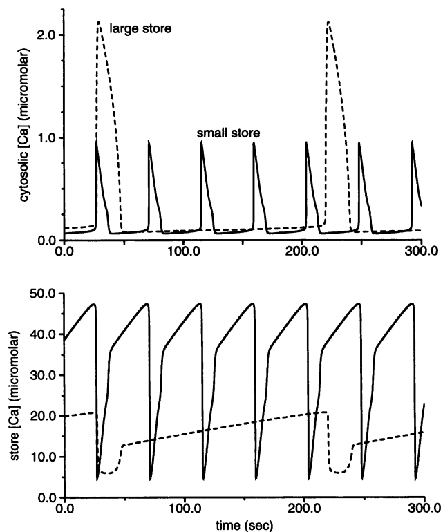
FIGURE 5 Oscillations in (top) [\text{Ca}_i^{2+}] and (bottom) [\text{Ca}_s^{2+}] for the open-cell model; (—) Small internal store, (---) large internal store; other parameters are given in Table 3.
