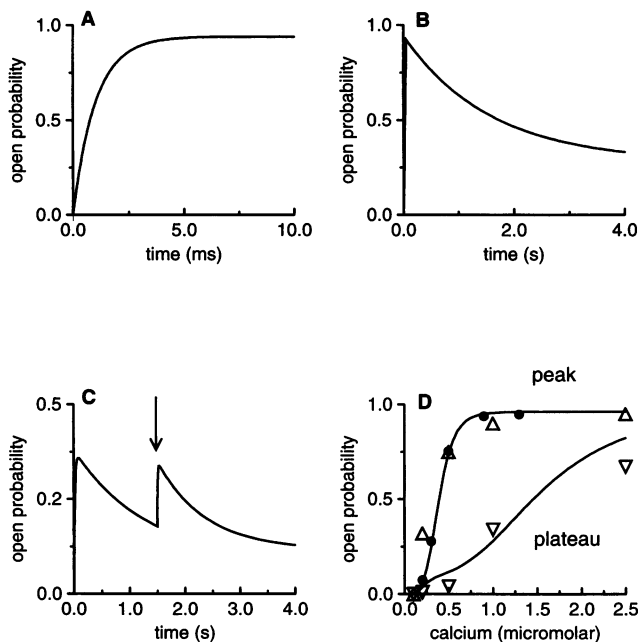
FIGURE 2 (A) Simulation of the rapid rise to the peak open probability of a single RyR following an increase of [Ca 2+ ] from 0.1 to 0.9 μM, calculated with Eqs. 1–4 and the rate constants in Table 1. (B) Same as (A) but on a longer time scale to show the decline to the plateau open probability. (C) Same as (B) but with two increases in [Ca 2+ ]: from 0.1 to 0.35 μM at t = 0 followed by an increase to 0.50 μM at the arrow. Note the adapted response. (D) The peak and the plateau open probabilities as functions of [Ca 2+ ]. (Solid curves) Theoretical values from Eqs. 15 and 16; (●) simulations like that in (A); (Δ) Experimental data (Fig. 2 B of Györke and Fill, 1993) (upward facing triangles are the peak; and downward, the plateau).
