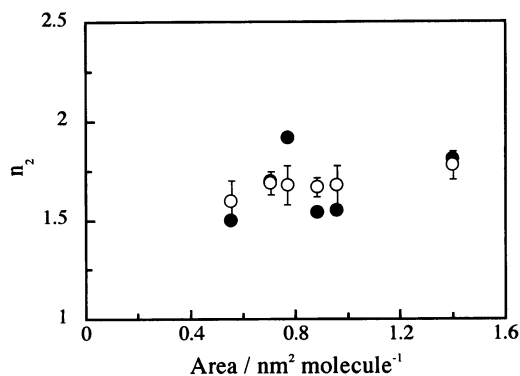
FIGURE 5 Change in the refractive indices n_{2p} (○) and n_{2s} (●) of the chlorophyll a monolayer with monolayer compression.
