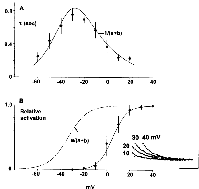
FIGURE 4 (A) Time constants as obtained by the procedure illustrated in Fig. 3. The error bars indicate mean \pm SD ( n = 6 ). The bell-shaped curve labeled 1/(a+b) corresponds to a = 0.9 \exp(0.04(V + 25)) \text{ s}^{-1} and b = 0.31 \exp(0.08(V + 25)) \text{ s}^{-1} . (B) Steady-state activation curve obtained from normalization of tail currents at -40 mV after steps to potentials indicated on the abscissa. An illustration of these results is given in the inset (calibrations are 0.5 s and 0.1 nA). The maximum, saturating tail current amplitude was used to normalize tail currents for all voltage steps. The results of this procedure for six preparations are shown. The dashed curve corresponds to (a+b)^{-1} , where a and b are given in (A). The solid curve corresponds to (1 + \exp(0.0017(V - 5)))^{-1} .
