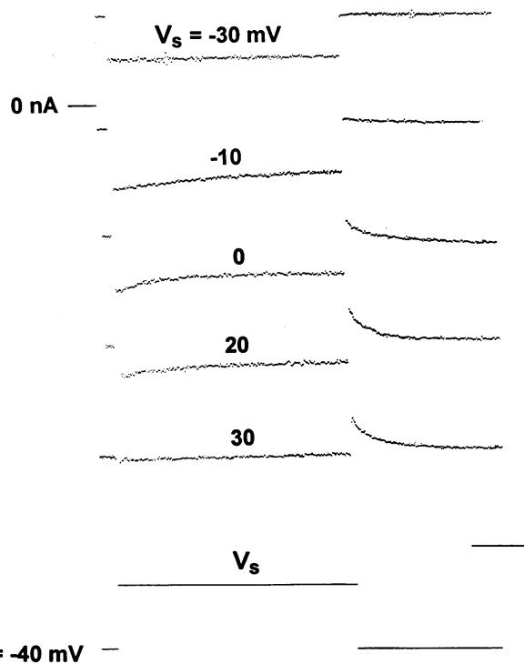
FIGURE 1 Membrane current measurements elicited by voltage steps to the potentials indicated above each record from a holding potential of –40 mV. The steady-state holding current was 0.22 nA, as indicated by the relationship between baseline current and the 0 nA mark for the –30 mV result. A similar relationship holds for the other records as well. The result for +30 mV was taken from a different preparation than the other four results. Calibrations are 0.5 s and 0.1 nA.
