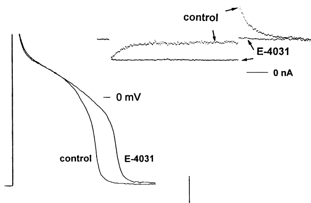
FIGURE 7 Effects of E-4031 ( 1 \mu M ) on the action potential waveform and on membrane current. (Inset) holding potential = -40 mV; step potential = +20 mV. The calibrations represent 100 ms and 25 mV for the action potentials, and 0.5 s and 0.1 nA for the membrane current results in the inset.
