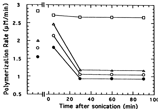
FIGURE 5 Time course of oxidized actin filament annealing after sonication. 0.5-ml aliquots of 12 \mu\text{M} G-actin solutions, previously treated with 0 mM ( \bullet , control), 5 mM ( \circ ), 10 mM ( \Delta ), and 20 mM ( \square ) \text{H}_2\text{O}_2 as described for Fig. 2, were incubated for 24 h in the presence of polymerizing salts (see Materials and Methods) and then sonicated (50 W for 5 s). At 5, 30, 60, and 90 min after disruption, 1.5 ml of 12 \mu\text{M} G-actin (10% pyrene-actin) was added to the sonicated F-actin samples. The rates of nucleated actin polymerization ( \mu\text{M min}^{-1} ) were calculated as indicated for Fig. 4 and were plotted versus time after sonication. The rates of nucleated polymerizations, before the mechanical fragmentation of F-actin "seeds," have been considered to reflect the steady-state concentration of growing ends in control and oxidized actin samples.
