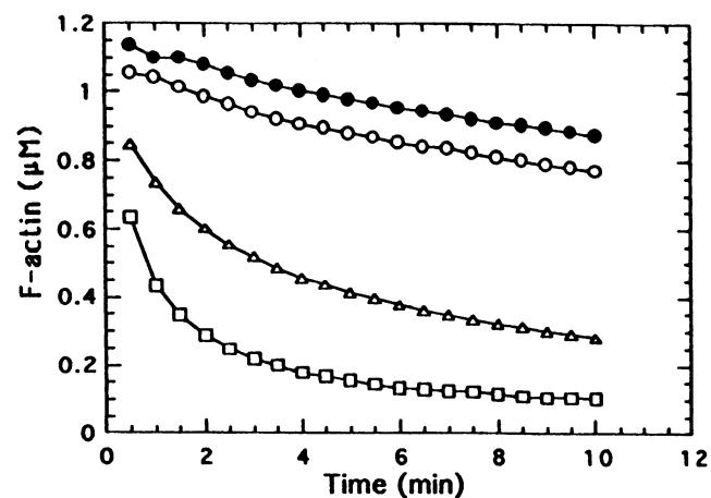
FIGURE 7 Depolymerization rate of oxidized actin filaments. 0.2-ml aliquots of 12 \mu\text{M} G-actin (20% pyrene-actin), previously incubated with 0 \text{ mM} ( \bullet , control), 5 \text{ mM} ( \circ ), 10 \text{ mM} ( \triangle ), and 20 \text{ mM} ( \square ) \text{H}_2\text{O}_2 as described for Fig. 2, were polymerized in test cuvettes. After 24 h incubation, depolymerization was initiated by diluting the oxidized F-actin samples tenfold with G-buffer (see Materials and Methods). The final concentrations of polymerizing salts in the assay were 10 \text{ mM} KCl and 0.2 \text{ mM} \text{MgCl}_2 . The maximum depolymerization rate was 0.033 \mu\text{M} \text{ min}^{-1} for control actin, and 0.046 , 0.19 , and 0.4 \mu\text{M} \text{ min}^{-1} for actin treated with 5 , 10 , and 20 \text{ mM} \text{H}_2\text{O}_2 , respectively.
