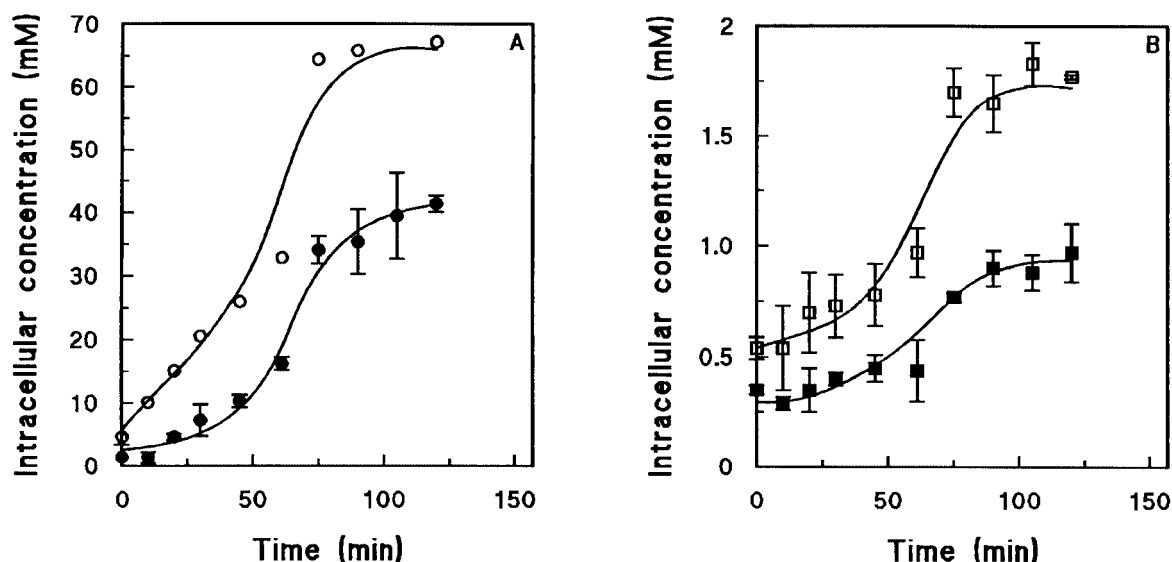
FIG. 5. Intracellular metabolite levels during anaerobic maltose fermentation by maltose-pregrown cells of S. cerevisiae EB.VW.4000 ( \Delta hxt1 through -17 \Delta gal2 \Delta agt1 \Delta YDL247w \Delta YJR160c ). (A) Symbols: \circ , maltose; \bullet , glucose. (B) Symbols: \square , glucose 6-phosphate; \blacksquare , ATP. Most of the values are averages \pm mean deviations for two experiments performed with cells from independent chemostat cultures; the only exceptions are the maltose values, which are values from a single experiment.
