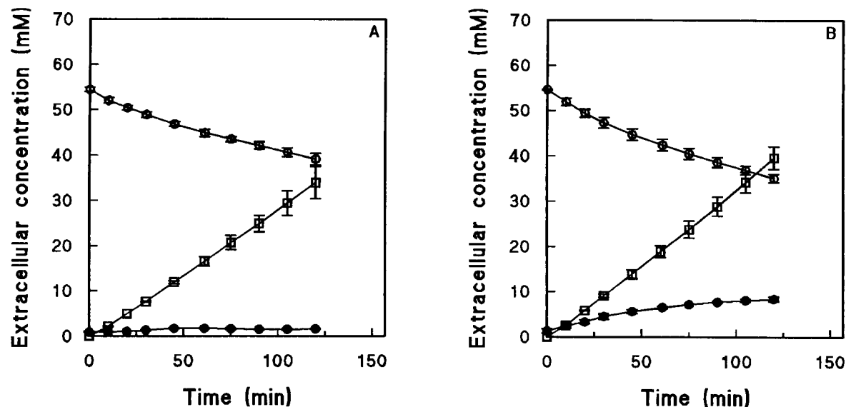
FIG. 4. Anaerobic fermentation of maltose by cells harvested from aerobic, maltose-limited chemostat cultures of S. cerevisiae EBY.VW.4000 ( \Delta hxt1 through -17 \Delta gal2 \Delta agt1 \Delta YDL247w \Delta YJR160c ) (A) and S. cerevisiae CEN.PK2-1C (reference strain) (B). Extracellular concentrations of maltose (○), glucose (●), and ethanol (□) are shown. The values are averages \pm mean deviations for two experiments performed with cells from independent chemostat cultures.
