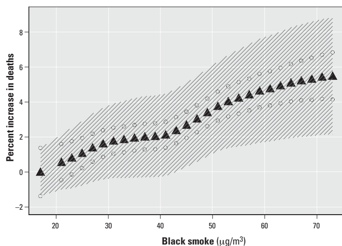
Figure 2. The metasmoother of the concentration–response relation between black smoke and daily deaths (on a percent scale). Each triangle represents the meta-analysis of the estimated effect in that 2\ \mu\text{g}/\text{m}^3 increment in exposure from each of the eight cities, incorporating a random variance component. The shaded lines denote the pointwise 95% CI for each estimate. The circles show what the 95% CI would have been had a random variance component not been estimated. The difference indicates the increased variance in the estimate due to heterogeneity among the cities in the response to particles. The association is essentially linear across its entire range.
