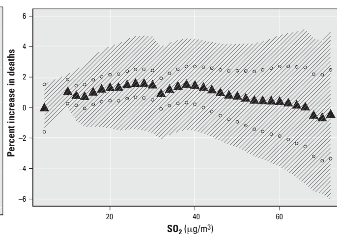
Figure 3. The metasmoother of the concentration–response between \text{SO}_2 and daily deaths (on a percent scale). Each triangle represents the meta-analysis of the estimated effect in that 2\ \mu\text{g}/\text{m}^3 increment in exposure from each of the eight cities, incorporating a random variance component. The shaded lines denote the pointwise 95% CI for each estimate. The circles show what the 95% CI would have been had a random variance component not been estimated. The difference indicates the increased variance in the estimate due to heterogeneity among the cities in the response to \text{SO}_2 . There is little evidence of a causal concentration–response relation.
