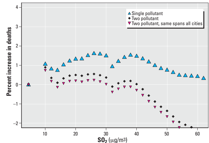
Figure 7. The concentration–response between \text{SO}_2 and daily deaths in a single-pollutant model, a two-pollutant model, and a two-pollutant model with an alternative specification of the season and weather model that did not vary across cities.
