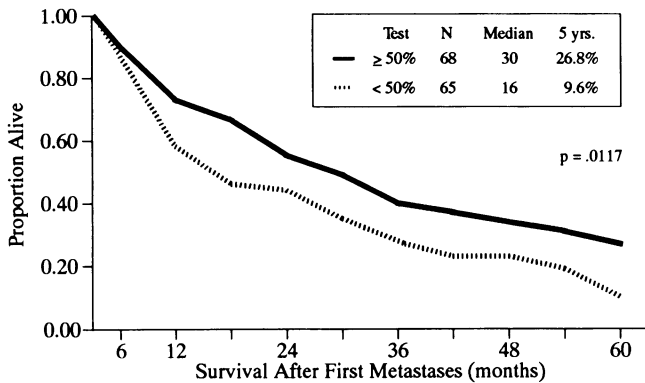
FIG. 1. Correlation between IgM antibody response and survival in patients with advanced-stage melanoma who were receiving active immunotherapy. Five-year survival rate 26.8% versus 9.6%.
