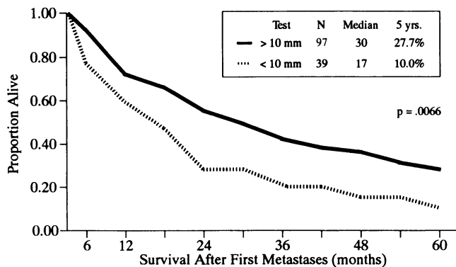
FIG. 2. Comparison of the response to MCV skin tests and survival in advanced-stage melanoma. Five-year survival rate 27.7% versus 10%.
