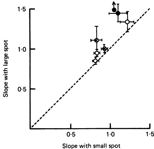
Fig. 6. A comparison of the slopes of the log increment threshold-log background intensity lines obtained with the 1.9 mm and the 0.3 mm stimuli from seven cells. The slopes are regression coefficients calculated on the basis of the data points lying between 5 and 9 log units background intensity. The bars give the standard deviations of the coefficients. ●, refer to sustained cells; ○, to class 3 cells and ⊕, to cells not classified.
