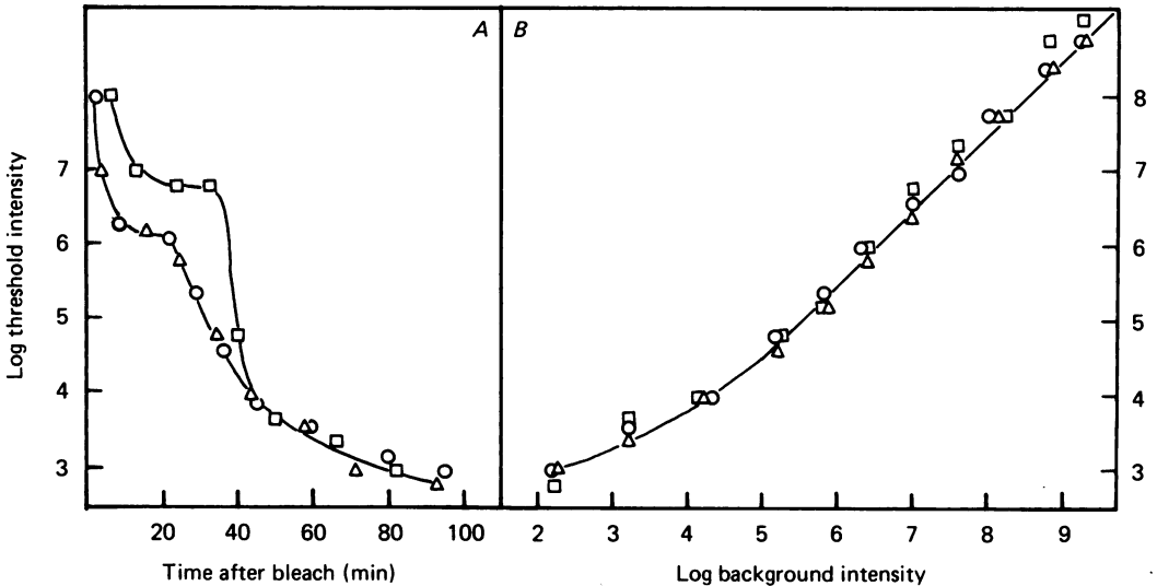
Fig. 5. The different effects of bleaching adaptation and background adaptation on threshold. The threshold of a class 3 cell was first followed after a full-field 3% bleach (A), then against successively increased 558 nm full-field backgrounds (B). Stimuli were 513 nm spots with diameters 0.3 mm (○), 0.8 mm (△) and 1.9 mm (□). When the increment thresholds against backgrounds had been measured, the retina was bleached anew and it was ascertained that the differences did not depend on some general deterioration of the inhibitory mechanism. The central summation area of the receptive field had a diameter of 0.3 mm in the dark-adapted state.
