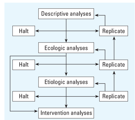
Figure 1. Decision tree for statistical framework.
