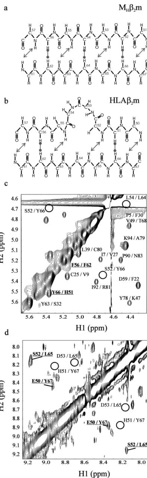
Fig. 3. Schematic diagram showing the pattern of NH–NH and C \alpha H–C \alpha H NOEs predicted for conformations of M H \beta 2 m (a) lacking and (b) containing the \beta bulge involving residues 53 and 54. C \alpha H–C \alpha H region (c) and NH–NH region (d) of a 1 H– 1 H NOESY spectrum of M H \beta 2 m acquired at pH 5.7, 37°C, in D 2 O and H 2 O, respectively. Crosspeaks consistent with the presence of the \beta bulge in solution are marked in bold and underlined. Crosspeaks expected were M H \beta 2 m to adopt a conformation in solution identical to that in a are shown as solid circles.
