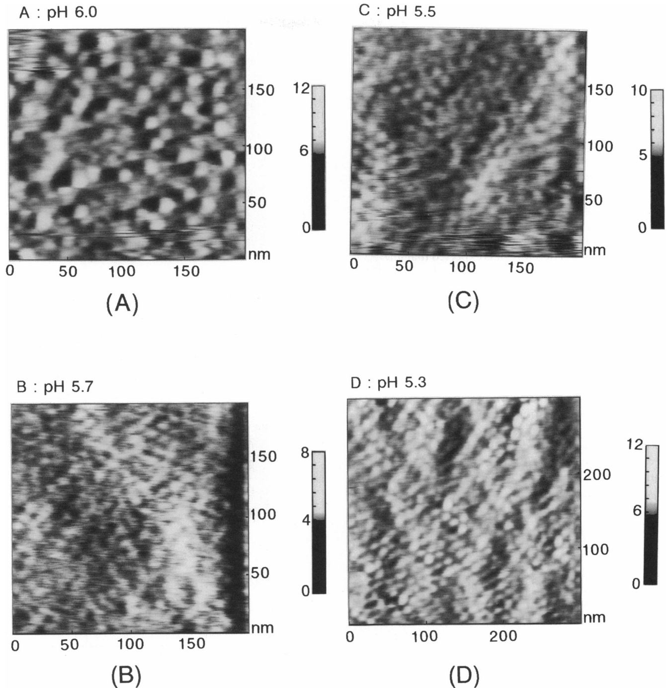
FIGURE 2 Unfiltered AFM images of ferritin samples prepared at pH: (A) 6.0; (B) 5.7; (C) 5.5; and (D) 5.3. The image area is: (A–C) 200 \times 200 \text{ nm}^2 ; and (D) 300 \times 300 \text{ nm}^2 . The imaging was carried out in pure water.
