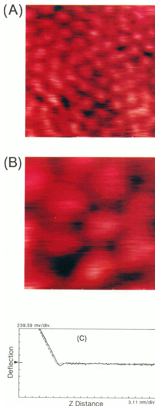
FIGURE 1 (A) Unfiltered AFM image of a regular array of ferritin molecules bound to a PBLH layer on a silicon wafer. The imaging was carried out in pure water using a fluid cell. Image area is 125 \times 125 nm 2 . (B) Higher magnification AFM image showing a hexagonal packing of ferritin molecules. Image area is 45 \times 45 nm 2 . (C) Force curve for Fig. 1 A. Cantilever deflection in millivolts ( ordinate ) versus distance between stylus and sample in nanometers ( abscissa ). The two curves are for approach ( dashed line ) and for withdrawal ( solid line ) of the stylus from the sample. Arrowhead (▶) indicates the operation point. It was estimated from this curve that the force applied was 10^{-10} N \sim 10^{-11} N.
