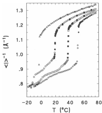
FIGURE 4 Inverse chain extension \langle l \rangle^{-1} versus T . \langle l \rangle^{-1} is obtained from M_1 using the relationship given in Eq. 4. ( \Delta ) DLPC- d_{46} , ( \circ ) DMPC- d_{54} , ( \square ) DPPC- d_{62} , ( \diamond ) DSPC- d_{70} . The open symbols are obtained from the data presented in Fig. 2. The solid symbols are additional data sets collected from the same samples or samples prepared in the same way from the same stock material in order to better localize the transition.
