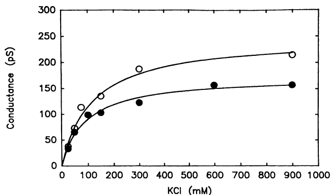
FIGURE 1 Single-channel conductance as a function of K^+ concentration for two different K^+ channels of the tonoplast of Chara . Measurements were done on inside-out excised-patches in symmetrical KCl concentrations. Data were fitted with the Michaelis-Menten equation. The single channel conductance was 90 pS (●) and 130 pS (○) in symmetrical 150 mM KCl.
