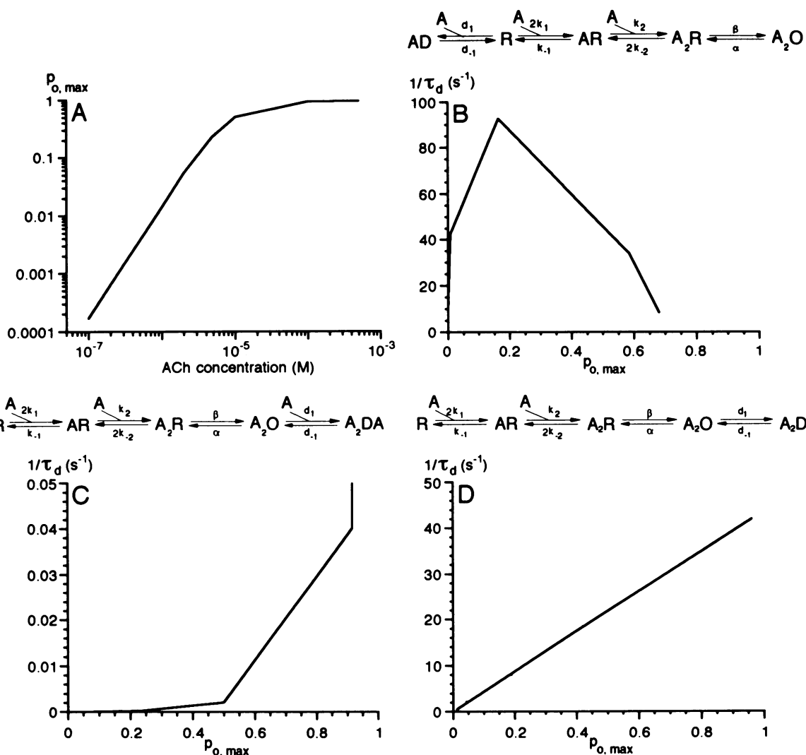
FIGURE 2 (A) Dose-response curve for the maximal probability of channel opening, p_{o, \max} , calculated for the reactions schemes in B, C, and D (the result was identical). (C–D) Plot of 1/\tau_d versus p_{o, \max} , calculated for the reaction schemes shown.
