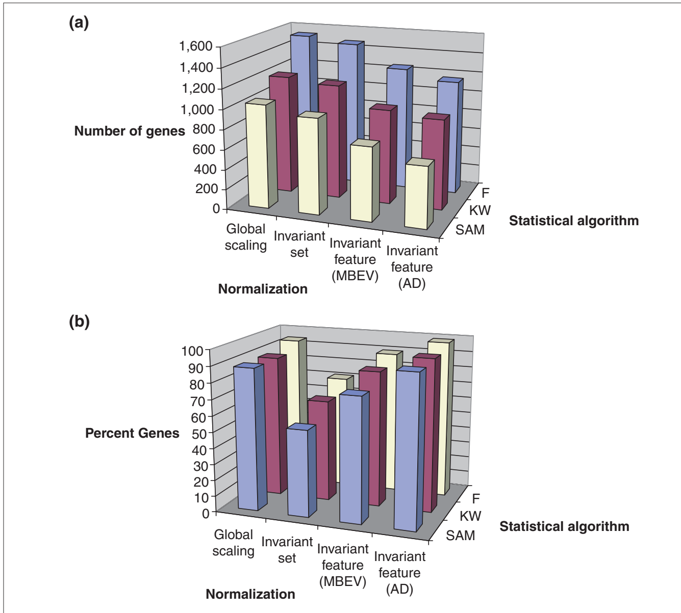
Figure 3 Results of testing different combinations of analysis methods. (a) Numbers of genes reaching a 99% confidence level in all possible combinations of normalization and statistical analysis algorithms. x-axis, normalization methods; y-axis, statistical analysis algorithms. Column height, number of genes. (b) Percentage of genes from Figure 2a that additionally reach a ratio of at least 2 and an absolute difference of at least 100 units. Layout is as in Figure 2a. AD, average difference; F, F-statistics; KW, Kruskal-Wallis; MBEV, model-based expression values; significance analysis of microarrays (SAM).
