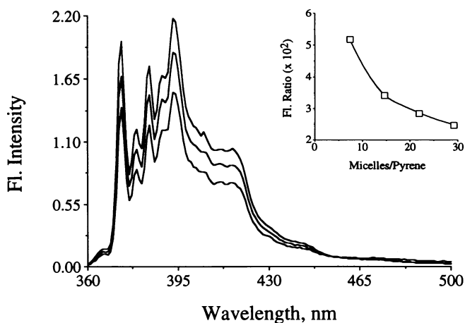
FIGURE 5 The fluorescence spectrum of pyrene in Tween 80 as a function of the micelle/pyrene ratio. 5.0 \mu\text{M} pyrene in Tween 80, 10 mM Mops, pH 7.2, excitation wavelength 337 nm. Lower spectrum obtained with 0.2% (wt/vol) detergent, middle spectrum obtained with 0.4%, upper spectrum obtained with 0.6%. The spectrum with 0.8% Tween 80 (not shown) was identical to that containing 0.6%. (Inset) The ratio of pyrene fluorescence intensity at 470 nm to that at 393 nm vs. the ratio of Tween 80 micelles/pyrene. The actual micelle/pyrene ratio used in the n_{\text{agg}} determination for this detergent was 36.
