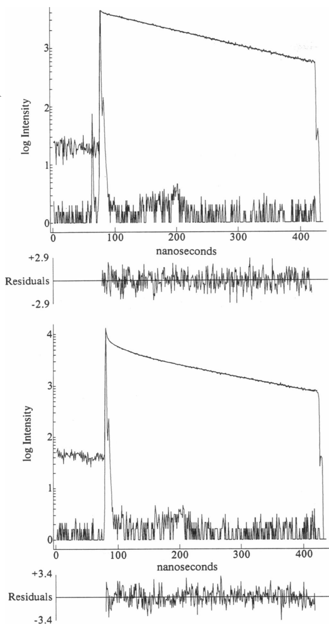
FIGURE 4 The fluorescence decay of 10 \mu\text{M} pyrene in 1.0% (wt/vol) reduced Triton X-100, 10% (vol/vol) ethanol, 10 mM Mops, pH 7.2, in the absence and presence of coumarin 153. Excitation wavelength 321 nm, emission wavelength 380 nm. (Top) Without C153. A three-exponential decay fits the data; A_1 = 0.207 , T_1 = 2.45 ns, F_1 = 0.004 , A_2 = 0.026 , T_2 = 55.5 ns, F_2 = 0.011 , A_3 = 0.767 , T_3 = 176 ns, F_3 = 0.986 , and \chi^2 = 1.03 . (Bottom) With 100 \mu\text{M} coumarin 153. A three-exponential decay fits the data; A_1 = 0.661 , T_1 = 2.08 ns, F_1 = 0.033 , A_2 = 0.137 , T_2 = 26.0 ns, F_2 = 0.085 , A_3 = 0.202 , T_3 = 181 ns, F_3 = 0.882 , and \chi^2 = 1.18 . The residuals are the difference between the theoretical fit and the data, divided by the square root of the data.
