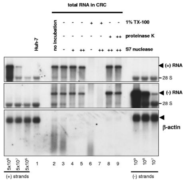
FIG. 4. Quantification of nuclease-resistant HCV positive- and negative-strand RNA and \beta -actin mRNA in CRCs. Total RNA equivalent to 5 \mu l of CRCs treated with 1% Triton X-100, 0.8 (+) or 8 (++) mg of proteinase K/ml and/or 0.2 (+) or 2 (++) U of S7 nuclease/ \mu l for 60 min at 25°C or from mock-treated CRCs, as indicated on top, was subjected to Northern hybridization analysis with a negative-strand riboprobe to detect viral positive-strand RNA (top panel), a positive-strand riboprobe for HCV negative-strand detection (middle panel), and a riboprobe specific for the detection of cellular \beta -actin mRNA. The positions of viral positive- and negative-strand RNA and \beta -actin are indicated by arrowheads at the right. For quantification, in vitro transcribed replicons corresponding to known amounts of viral positive- and negative-strand RNA were mixed with 2 \mu g of total cellular RNA from naive Huh-7 cells and loaded as indicated at the bottom of the figure. We used 4 \mu g of total RNA from naive Huh-7 cells as a negative control (Huh-7, lane 1). We quantified the viral RNAs by phosphorimaging and found ca. 3 \times 10^6 negative-strand and 3 \times 10^7 positive-strand RNAs per \mu l of CRCs in this particular experiment.
