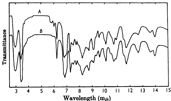
Fig. 4. Infrared spectra of \delta -tocotrienol (A) and \delta -tocopherol (B). Both compounds were examined as oily films.
