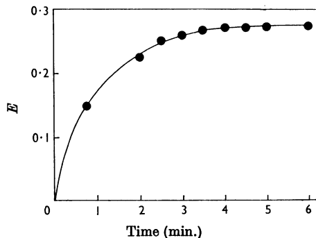
Fig. 6. Rate of colour production for \delta -tocotrienol with the Emmerie-Engel reagent. The \delta -tocotrienol concentration (in the reaction mixture) was 0.000493%.
