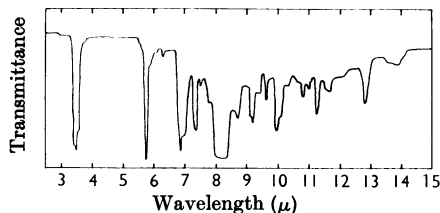
Fig. 8. Infrared spectrum of \delta -tocotrienyl ethyl carbonate. The sample was examined as an oily film.
