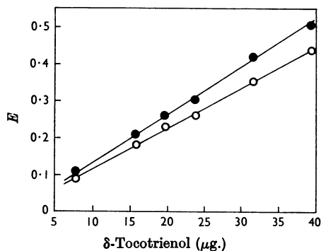
Fig. 5. Standardization graph for reaction between \delta -tocotrienol and the Emmerie-Engel reagent. \circ , Readings 2 min. after adding \text{FeCl}_3 ; \bullet , readings 3 min. after adding \text{FeCl}_3 .
