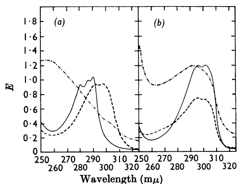
Fig. 2. Ultraviolet spectra of some fractions from chromatography of latex lipid on alumina. (a) \cdots , Light-petroleum fraction (0.042%); \text{—} , 2%-E/P fraction (0.036%); \text{---} , 4%-E/P fraction (0.035%). (b) \text{—} , 8%-E/P fraction (0.036%); \text{---} , 15%-E/P fraction (0.136%); \text{- - -} , diethyl ether fraction (0.180%).
