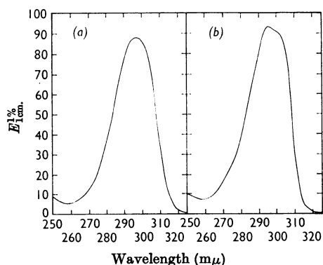
Fig. 3. Ultraviolet spectra of \delta -tocotrienol: (a) in ethanol; (b) in cyclohexane.
