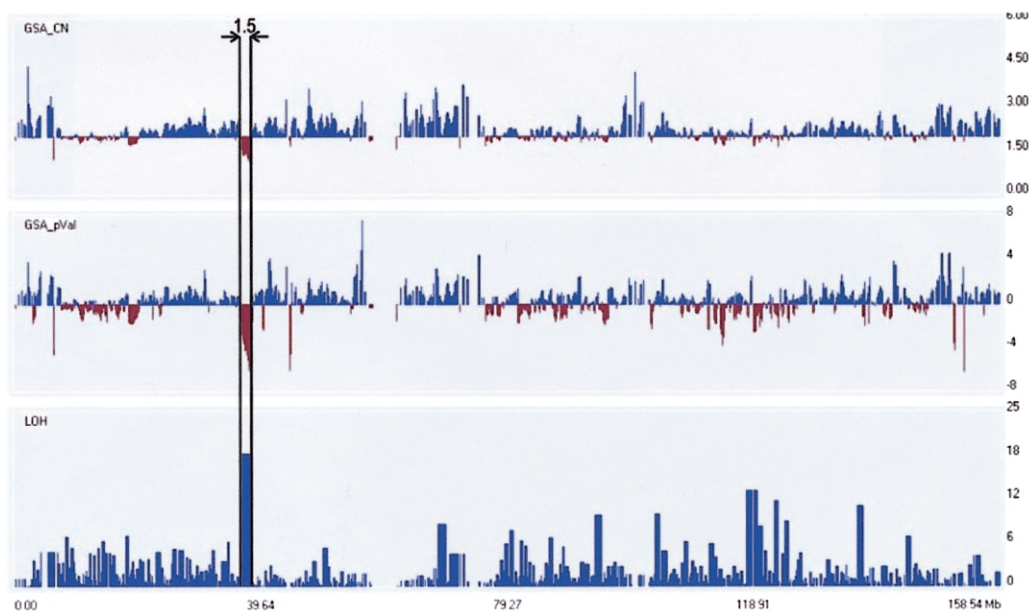
Figure 1 Analysis of Mapping 100K data with use of CNAT. Patient C1 is shown, with the 1.5-Mb deleted region on chromosome 7p14.1-14.2 indicated by vertical lines. Chromosomal position (in Mb) is indicated on the X-axis for all three panels. Estimated copy-number changes are shown in the upper panel, P values are shown in the middle panel, and the LOH score is shown on the bottom panel. The default window size of 0.5 Mb was used.
