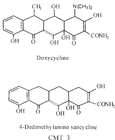
FIG. 1. Structures of doxycycline and CMT-3. Note that for CMT-3, the dimethylamino group at the A ring has been removed, resulting in the loss of antibacterial properties.
