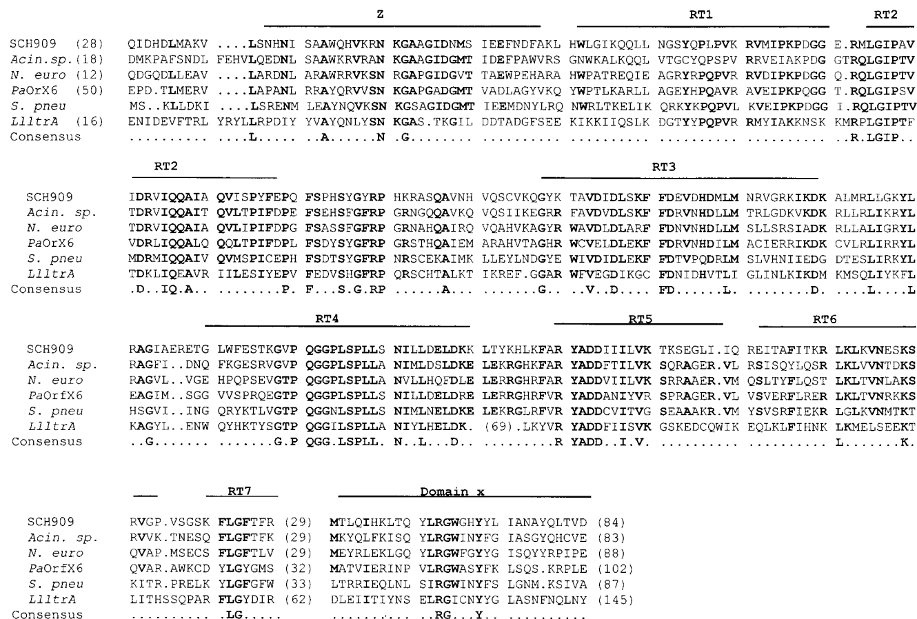
FIG. 2. Protein alignment of the putative maturase, Smtr, in SCH909 with eubacterial group II intron-encoded proteins from an Acinetobacter sp. ( Acin.sp. ) (J. H. Yum et al., unpublished; GenBank accession number AF369871; ORF II), N. europaea ( N. euro ) (JGI, unpublished), P. alcaligenes ( PaOrX6 ) (36), Streptococcus pneumoniae ( S. pneu ) (5), and Lactococcus lactis ( LlItrA ) (18). Consensus amino acids (four or more identical in the six sequences) are in bold letters. Domains conserved among intron-encoded proteins are denoted by the lines above the alignment. RT1 through RT7, RT-like domains (19); z, domain of undetermined function in non-long terminal repeat retroelements; x, maturase-specific domain (19). Numbers in parentheses indicate numbers of amino acids not shown.
