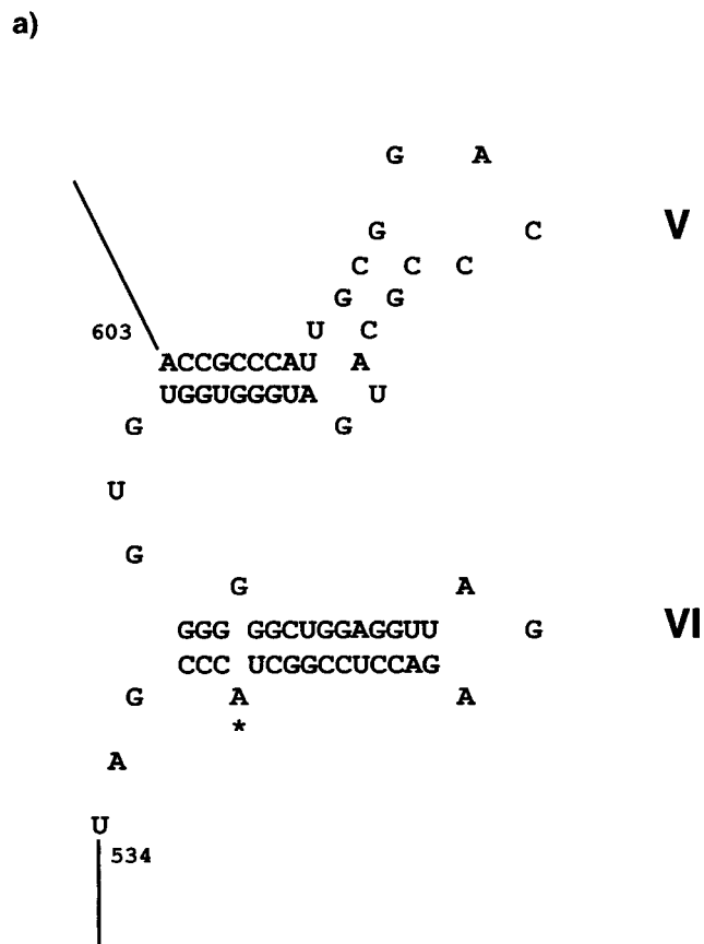
FIG. 3. General features of Smtr and its insertion site. (a) Secondary structure model of domains V and VI of the group II intron, Smtr, within integron 2 from SCH909. The boundary of the intron and the ant(2'')-Ia attC site is indicated by a vertical line. The bulging adenine residue involved in lariat formation is indicated by an asterisk. (b) Nucleotide sequence alignment of the ant(2'')-Ia stop codon and its attC site (59-base element) (4) with the ant(2'')-Ia gene and Smtr-intron boundary from SCH909). ant(2'')-Ia stop codons are indicated by asterisks. Exon sequences are shown in bold letters. (c) Nucleotide sequence alignment of the group II introns of SCH909 and N. europaea . The latter is adjacent to an attC site on one end; there is no recognizable ORF on the other end.
