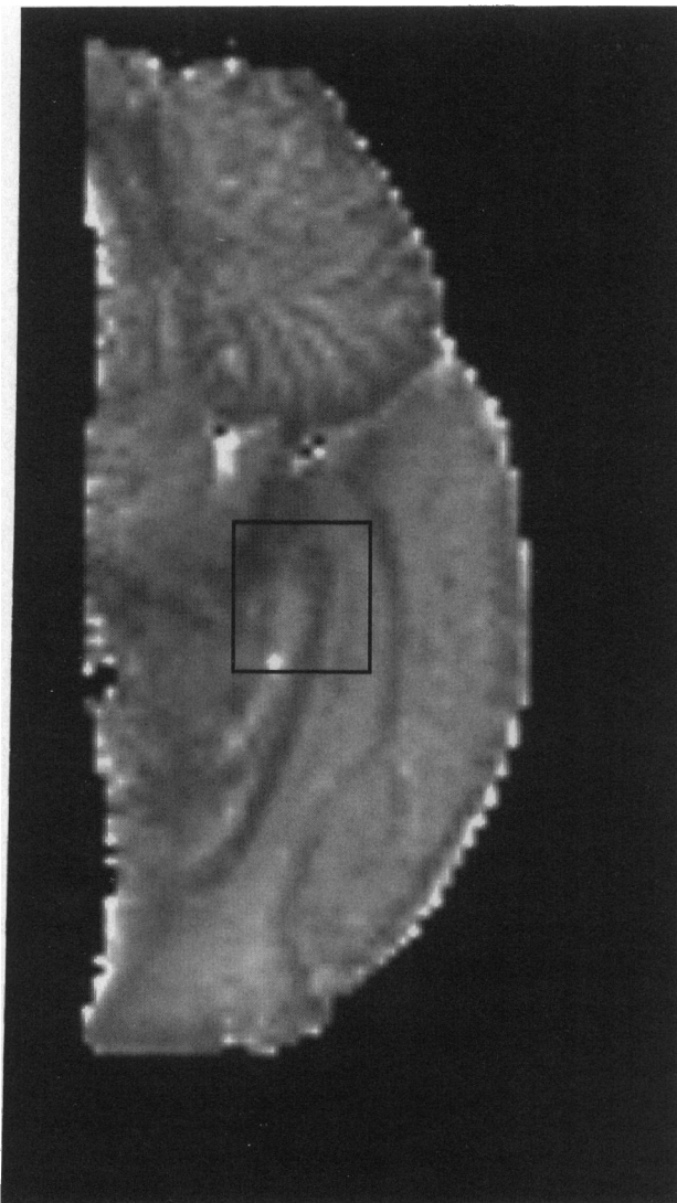
FIGURE 8 Image of \text{Tr}(\mathbf{D}_{\text{eff}}) , calculated for the sagittal section of excised cat brain shown in Fig. 6. The box indicates the ROI from which the diffusion ellipsoids were constructed in Fig. 7.
