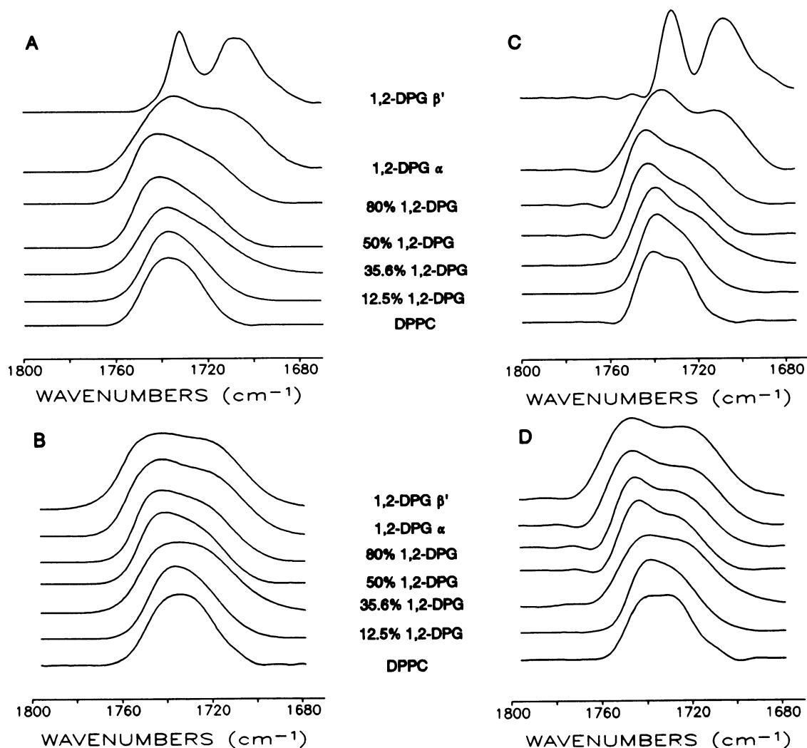
FIGURE 7 Infrared spectra in the region 1800–1670 cm -1 of pure DPPC, pure 1,2-DPG in both \alpha and \beta forms and different mixtures at 35°C (A, C) and 70°C (B, D), as indicated. The deconvoluted spectra for the 35 and 70°C original spectra are shown in C and D, respectively.
