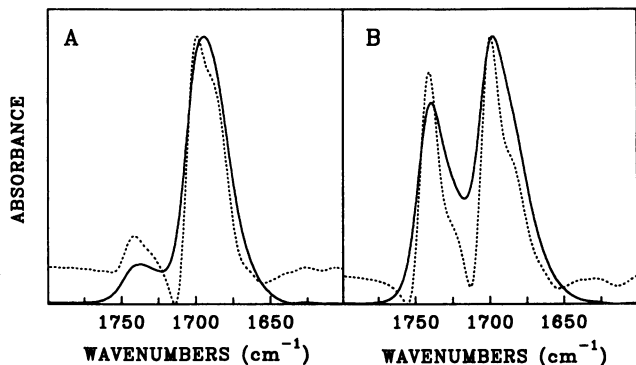
FIGURE 8 Infrared spectra recorded of an aqueous dispersion of (A) pure [sn-1,2-1- 13 C]-DPPC and (B) a mixture of [sn-1,2-1- 13 C]-DPPC plus 35.6 mol% of 1,2-DPG recorded at 35°C in the region 1800–1600 cm -1 . Broken lines show spectral deconvolutions.
