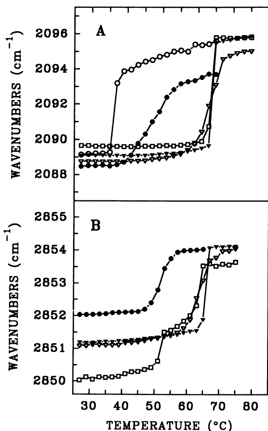
FIGURE 6 Temperature dependence of the frequency of the symmetric \text{C}^2\text{H}_2 (DPPC- d_{62} ) stretching (A) and symmetric \text{CH}_2 (1,2-DPG) stretching (B) of pure DPPC- d_{62} (○), and mixtures of DPPC- d_{62} containing 12.5 mol% (●), 35.6 mol% (▽), 50 mol% (▼), and 80 mol% (□) of 1,2-DPG.
