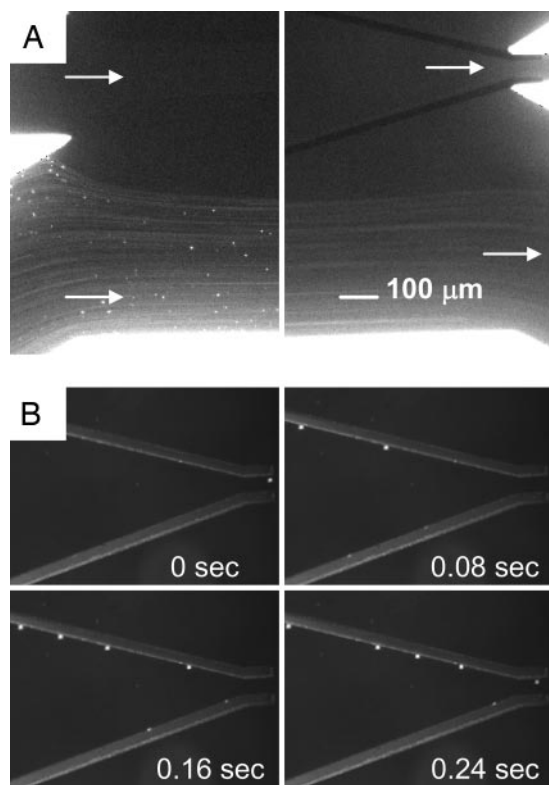
Fig. 2. Optical micrographs of the stabilized flow at the inlet and outlet channels. (A) The unlabeled cells follow the streamline and enter the waste channels, and the diffusion of the cells into the buffer stream is minimal. (B) Sequentially captured images of polystyrene beads moving under the influence of DEP deflection. Quadrupole electrodes guide the beads to the center of the microchannel. Total volume flow rate is 240 \mu\text{l/h} . Applied voltage is 20 V peak-to-peak at 500 kHz.
