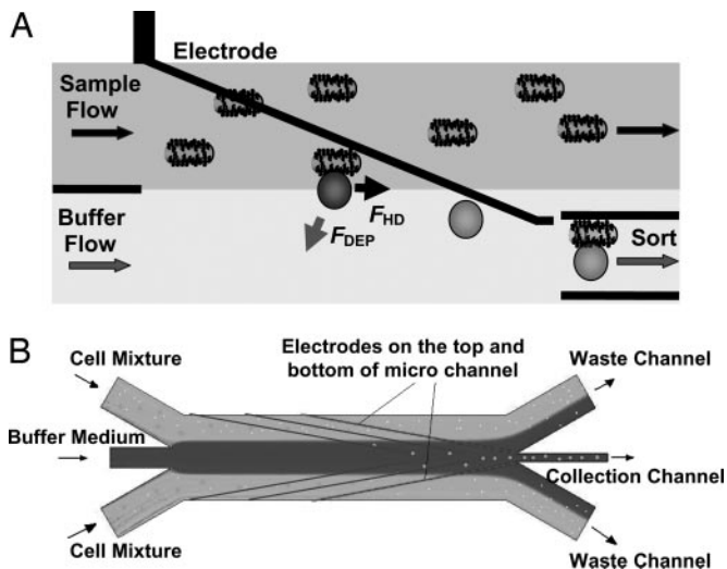
Fig. 1. Operational principle of DACS. (A) The DACS concept: Cells entering in the sample stream are only deflected into the collection stream if they are labeled with a dielectrophoretically responsive label. (B) Schematic view of the electrode region of the microchannels with sample and buffer inlets, as well as waste and collection outlets.
