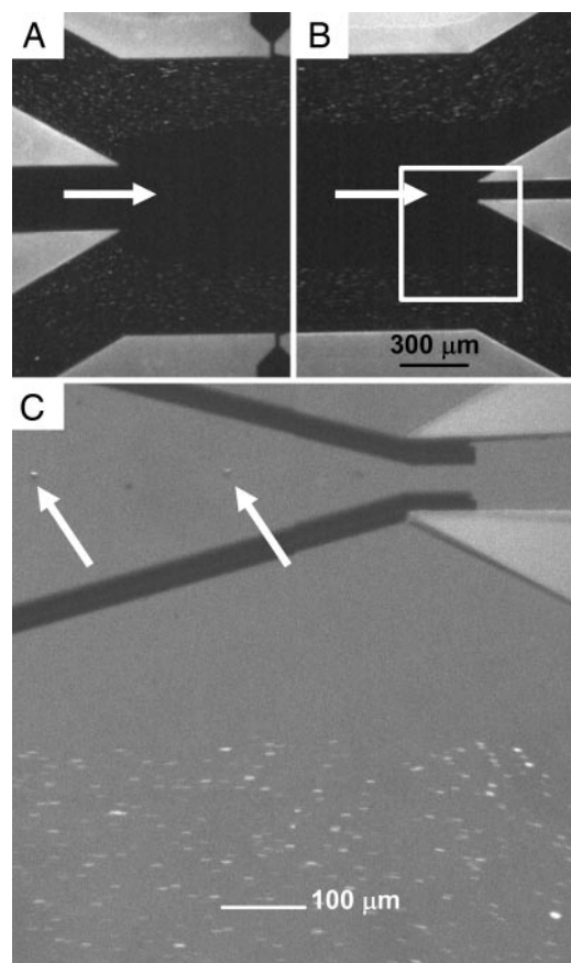
Fig. 3. Flow pattern of fluorescent cells in the DACS device. (A and B) Optical micrographs of streaming E. coli cells at the inlet (A) and outlet (B) channels. (C) An expanded view using optical microscopy, showing DEP particles entering the collection channel after being focused into the center of the stream. The arrows identify two beads carrying bound cells. Total volume flow rate is 300 \mu\text{l/h} , and the applied voltage is 20 V peak-to-peak at 500 kHz.
