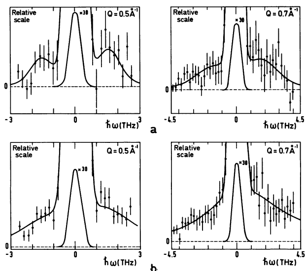
FIGURE 1 Scattered intensity I vs. \hbar\omega from constant- Q scans at Q = 0.5 \text{ \AA}^{-1} and Q = 0.7 \text{ \AA}^{-1} for a dry phycocyanin, (b) \text{D}_2\text{O} -hydrated phycocyanin. Full curves represent least-square fits according to a damped harmonic-oscillator model (compare reference Teixeira et al., 1985 for details). The typical \chi^2 values were \sim 1.3
