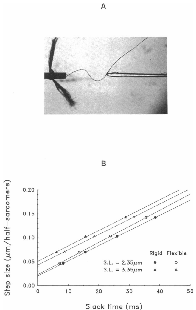
FIGURE 8 The effect of adding a flexible link. ( A ) Photograph of a tetanically contracting tibialis anterior fiber 2 ms after a step of 0.17 μm per sarcomere. Fiber is attached to motor wire via 2 mm of a single strand of silk. Note that the silk strand buckles while the fiber remains straight. Calibration bar indicates 1.0 mm. ( B ) Slack test plots. Adding the flexible link increased the intercept from 20.7 to 23.3 nm per half-sarcomere at the short length but decreased it from 51.3 to 43.4 nm per half-sarcomere at the long length. The range of V u values is 6% of the average value. S.L. , sarcomere length.
