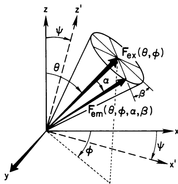
FIGURE 4 Optical arrangement for orientation-independent fluorescence anisotropy imaging. The excitation ( \mathbf{F}_{ex} ) and emission ( \mathbf{F}_{em} ) vectors of a single TMA-TPH fluorophore are shown. The coordinates \theta and \phi are referenced to the x, y, z axes. \alpha is the angle between \mathbf{F}_{ex} and \mathbf{F}_{em} . \psi is the angle between the z and z' axes in the x-z plane. See text for further explanation.
