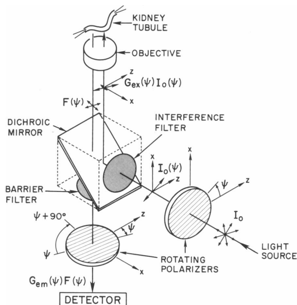
FIGURE 6 Optical path of the anisotropy imaging system containing rotatable excitation and emission polarizers. See text for explanation.
