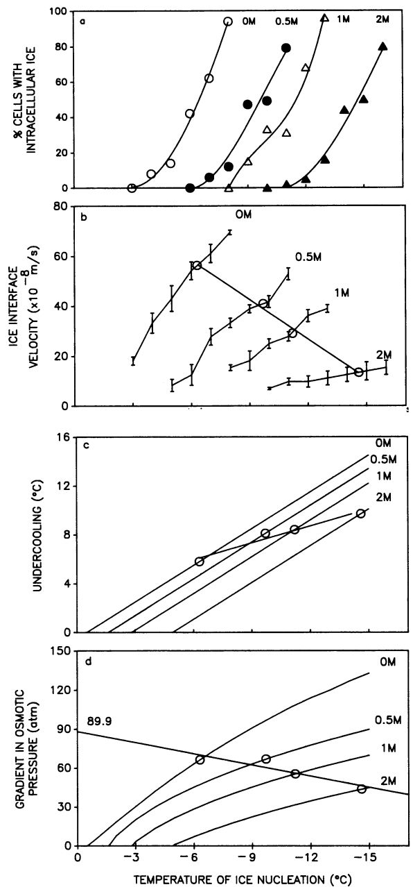
FIGURE 2 (a) Proportion of cells with intracellular ice after nucleation at various undercooled temperatures in four concentrations of glycerol. Seeding temperatures at which 50% of the cells freeze intracellularly are mapped onto b-d , and used as data points for regression analysis. The measured ice interface velocity for each condition is shown in b , where bars represent standard errors of three replicate measurements. The extent of undercooling on ice nucleation is shown in c , and the osmotic pressure gradient across the cell membrane on ice formation is shown in d . Slopes of the regression lines ( \pm SE) are as follows: (b) 5.23 \pm 0.34 ; (c) -0.46 \pm 0.068 ; (d) 2.88 \pm 0.95 .
